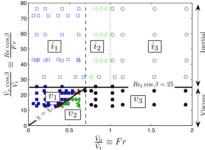
FIGURE 17. Classification of our results for the full range of simulations in the first and second regimes with laminar imposed flows: sustained back flow ( \blacksquare , \square ), stationary interface ( \blacktriangleright ), temporary back flow ( \blacktriangleleft , \triangleleft ) and instantaneous displacement ( \bullet , \circ ). Data point with filled symbols are viscous and with hollow symbols are inertial. The horizontal bold line shows the first order approximation to the inertial-viscous transition ( Re_t \cos \beta = 25 , from Fig. 10). The angled heavy line represents the prediction of the stationary interface from the two-layer lubrication model: \chi = \chi_c . The vertical dashed-line is \hat{V}_0/\hat{V}_t = 0.7 and the dotted-line is \hat{V}_0/\hat{V}_t = 1 . Regions marked with v_j and i_j ( j=1,2,3 ) are viscous and inertial, respectively, as explained in the main text.
