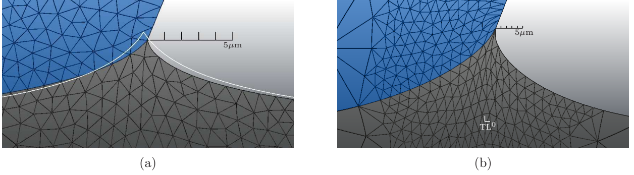
Figure 10: (a) Comparison between the nonlinear computation of the deformed configuration (coloured regions) and the linear analytical solution z = z_1(r) (white solid line) near TL in the the asymmetrical case ( \gamma_{12} \neq \gamma_{1V} ) for \delta = 0.01 . (b) Nonlinear computation of the deformed configuration for \delta = 0.07 and the cusp rotation.
