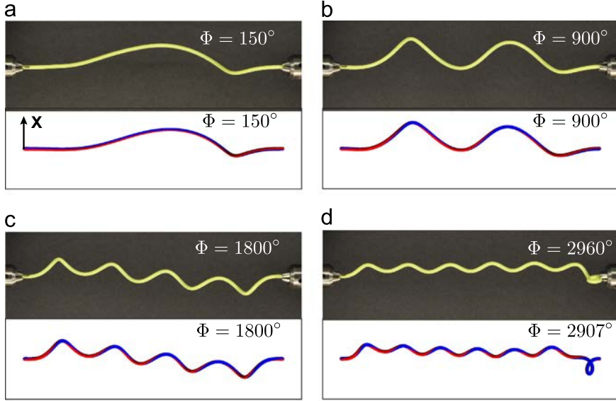
Fig. 10. Top view of various equilibrium configurations of a curly elastic rod ( \hat{\kappa}_1(s) = 44.84 \text{ m}^{-1} ) for increasing values of the rotating angle, \phi . The experimental pictures have a black background and the simulations have a white background. The simulation results are rendered to visualize twist by using bi-color rods. (a) Asymmetric out-of-plane equilibrium shape for \phi = 150^\circ , (b) one-twist-per-wave configuration for \phi = 900^\circ with three wavelengths between the two clamps, (c) one-twist-per-wave configuration for \phi = 1800^\circ with five wavelengths between the two clamps and (d) onset of formation of a plectoneme state at one extremity of the rod.
