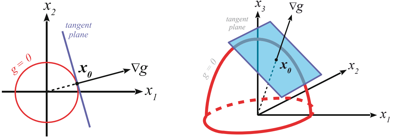
Figure 8. Tangent planes in 2D and 3D
