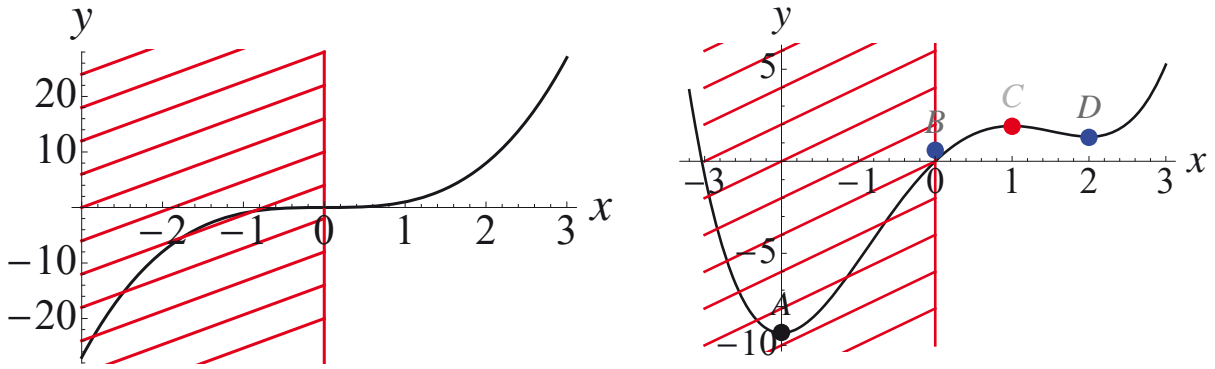
Figure 9. (Left) The function V(x) = x^3 with the constraint x \geq 0 . (Right) The function V(x) = \frac{1}{4}x^4 - \frac{1}{3}x^3 - 2x^2 + 4x with the constraint x \geq 0 . Points B and D are local minima, point C is a local maximum, and point A is a forbidden minimum.
