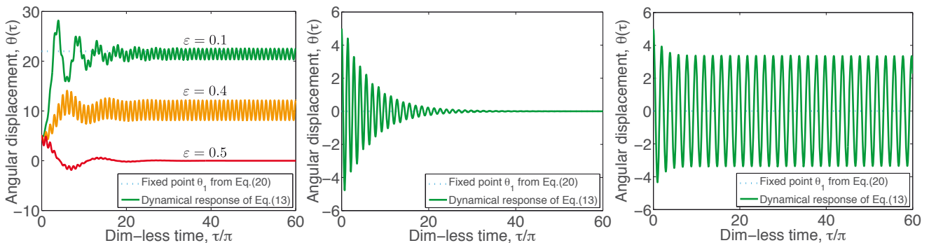
Figure 21. Temporal evolutions for \theta(\tau) , solution of Eq. (87), for initial conditions \mathbf{x}(0) = \{5^\circ, 0\}^T , Q = 20 and \beta = 1 . (Left) Dynamical response for p = 1.025 (that is \delta = -0.1 ) and various \varepsilon = [0.1, 0.4, 0.5] . (Center) Dynamical response for p = 0.5 (that is \delta = 2 ) and \varepsilon = 0.1 . (Right) Dynamical response for p = 0.75 (that is \delta = 1 ) and \varepsilon = 0.1 .
