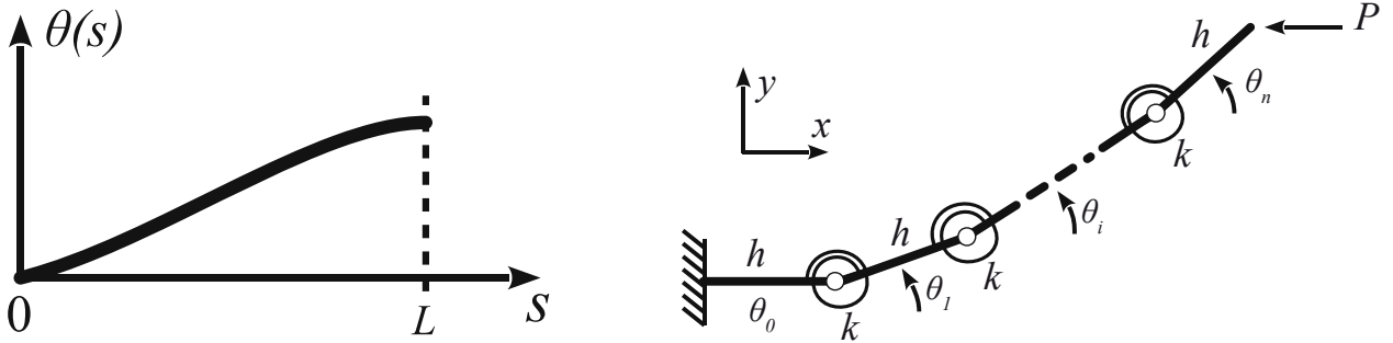
Figure 3. (Left) Solution \theta(s) for the configuration in Figure 2-Left. (Right) A system of rigid bars linked by spiral springs.
