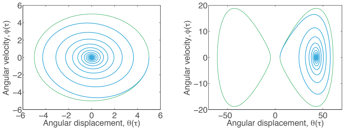
Figure 20. Dynamical response of Figure 19 in the phase plane (\theta(\tau), \phi(\tau)) . (Left) Trajectory for p = 0.75 and \mathbf{x}(0) = \{5^\circ, 0\}^T . (Right) Trajectories for p = 1.025 and \mathbf{x}(0) = \{5^\circ, 0\}^T or \mathbf{x}(0) = \{-5^\circ, 0\}^T .
