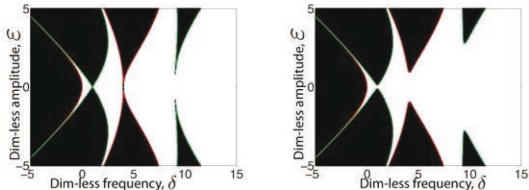
Figure 23. Mathieu's tongues or stability charts of the vertical solution of the system of Figure 16, in the (\delta, \varepsilon) plane. Unstable regions are in black. Regions bounded by green and red lines respectively lead to 2T and T -periodic steady-state oscillations. (Left) Undamped system with Q = 10^{10} , and (Right) Damped system with Q = 20 .
