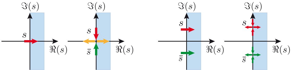
Figure 18. Stability of an equilibrium in the Argand plane. (Left) Static instability or instability by divergence can happen by simple crossing or locking of eigenvalues on the real axis. (Right) Dynamic instability or flutter instability can happen by crossing or locking of eigenvalues away from the real axis.
