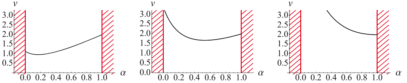
Figure 27. Graphs of the function (113) for (Left) \epsilon = 1.5 , (Center) \epsilon = 2.6 , (Right) \epsilon = 4 , where v'(1) = 0 .
