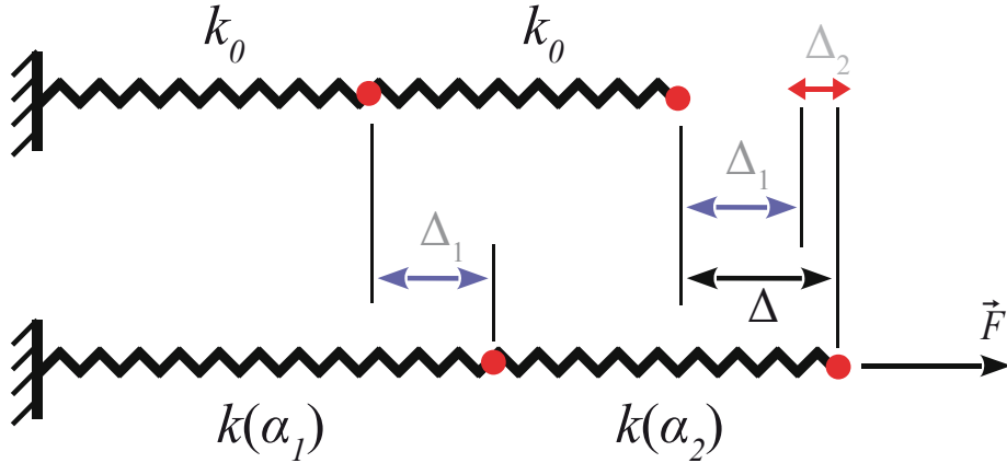
Figure 30. Two damageable springs in series. A displacement \Delta is imposed through to application of a tension F . During the loading procedure each spring may experience damage and have its stiffness k modified.
