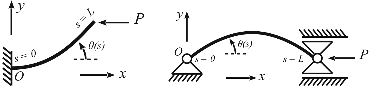
Figure 2. Elastic beams buckling in the plane. (Left) Clamped-free boundary conditions. (Right) Pinned-pinned boundary conditions.
