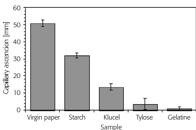
8 Water capillary ascension lengths on the papers impregnated with the different adhesives. All solutions used to impregnate the paper were prepared at the same concentration (5 % w/v). The adhesive concentrations (w/w) deposited in the paper: starch, 6.8 %; Klucel, 5.3 %; Tylose, 8.6 %; Gelatine, 6.3 %. Ten measurements were performed for each adhesive and only the average was taken.
