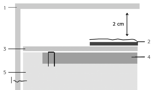
12 The framing of the artefact (cross section): Plexiglass® glazing (1); artefact mounted on the first (support) board (2); background board (3); honeycombed polycarbonate backboard stapled to the wooden frame (4); wooden frame (5).
