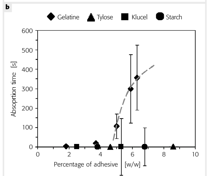
7 Absorption time of 1 ml drop of water against the percentage of adhesive deposited in the paper: Each value corresponds to an average of ten measurements performed on the side of the application (a), or on the side opposite to the application (b). Error bars correspond to standard deviations.
