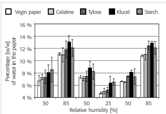
6 Water vapour absorption measurements at different humidity conditions. All solutions used to impregnate the paper were prepared at the same concentration (5 % w/v). The adhesive concentrations (w/w) deposited in the paper: starch, 5.8 to 7.7 %; Klucel, 6.3 to 8.5 %; Tylose, 6.5 to 8.4 %; Gelatine, 5.6 to 6.3 %.
