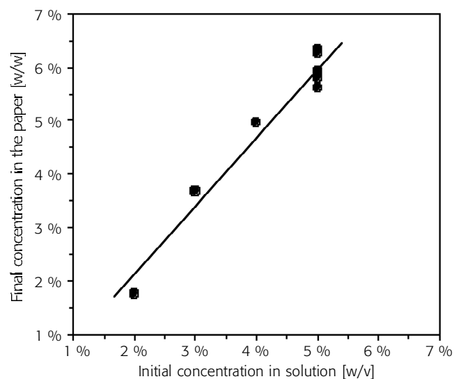
5 The gelatine content in the paper against the initial concentration in solution. The amount of gelatine impregnated in the paper is linearly correlated to the initial concentration in solution.
