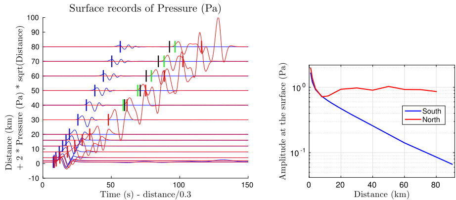
Fig. 14 On the left , simulated surface records sorted by distance (in km) as a function of reduced time (in s). Reduced time induces a shift of the records in the left direction by \text{Distance}/0.3 seconds to ensure a better readability of the figure. The amplitude of the records is scaled according to the formula provided in y-axis label for the same reason. Rays theoretical arrival times for direct waves are indicated by thick blue and red tags. The arrival times of rays reflected back to the surface at the top of the waveguide are indicated both for computations in Cartesian ( black tags ) and in spherical ( green tags ) geometry. On the right , maximum amplitude (in Pa) measured on simulated records as a function of distance to the source (in km). North (resp. South) stations are indicated in red (resp. in blue )
