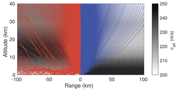
Fig. 13 Ray trajectories in the North ( left ) to South ( right ) plane at 240° solar longitude and 0 h local time. The background color scale indicates effective sound velocity with black and white color indicating highest and lowest effective velocities respectively
