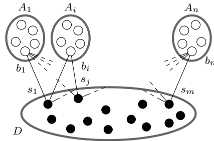
Figure 1: Schema of the constructed graph for the reduction from \mathbf{X3C} . The black and white nodes have latent profiles with values 1 and 0 respectively.
