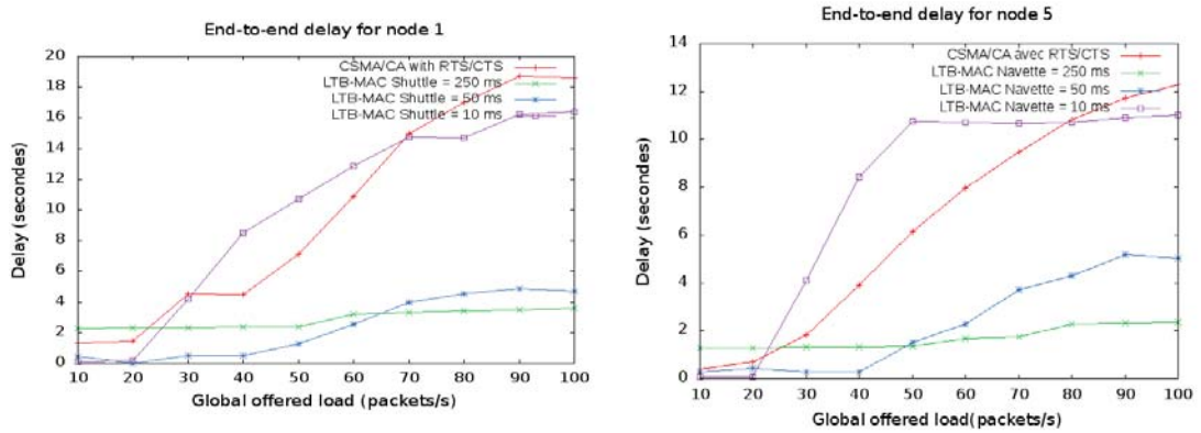
Fig. 8. End-to-end delay for node 1 and node 5
