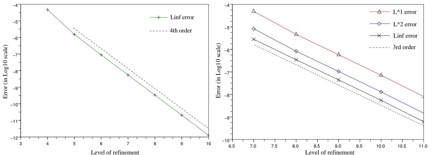
Figure 2: Test of convergence on non-uniform grids by means of accuracy doubling. The error is represented in log-scale amplitude. L^1 , L^2 and Linf label the errors measured with respect to the norms \|\cdot\|_{L^1} , \|\cdot\|_{L^2} and \|\cdot\|_{L^\infty} norms, and “4th order” and “3rd order” mean the functions f(h) = Ch^4 and f(h) = Ch^3 respectively. Left: test of the AMR Collatz solver. Right: test of the whole scheme, error on F(t = 10) .
