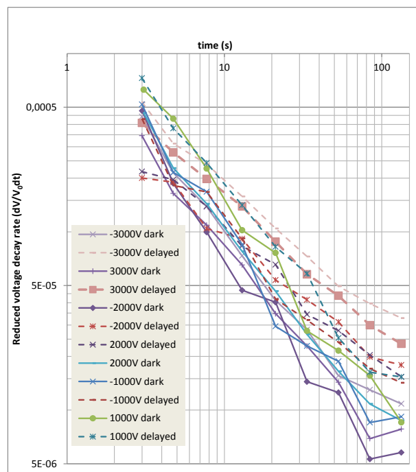
Figure 10. Voltage decay rates, in the dark before and after illumination 10 min blue LED illumination at the same initial voltage. Voltage rates reduced to the value of the initial voltage.
