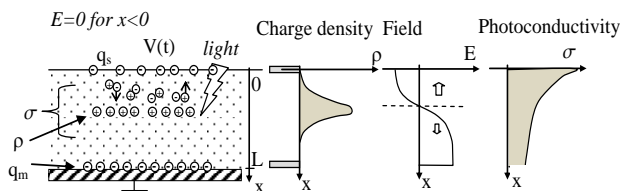
Figure 14. Return voltage under illumination
