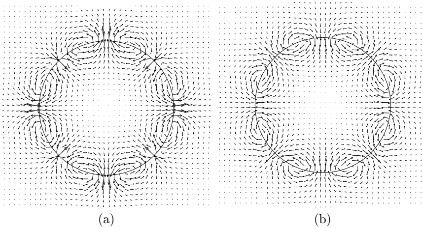
Fig. 9. Velocity fields at times (a) t \approx T_\lambda/4 and (b) t \approx 3T_\lambda/4 for La = \infty .
