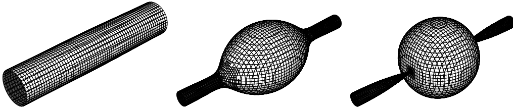
Fig. 19. Initial stages of a capillary jet instability: k r_0 = 0.628 , \epsilon = 0.02 , La = 238.34 . Physical parameters correspond to a jet of water in air. The non-dimensional times are from left to right 0, 11.32 and 12.1 (breakup time). The interface is represented using the VOF-reconstructed planar fragments in each cell.
