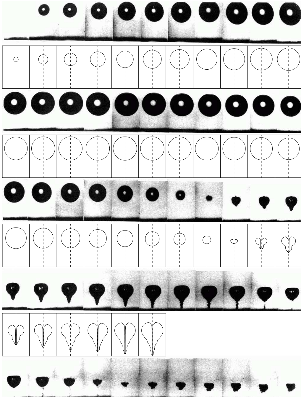
FIGURE 6. Comparison between a high-speed photographic series of a bubble collapsing near a wall (Lauterborn & Ohl 1997) and a direct numerical simulation. Sampling rate is 75 000 frames per second.
