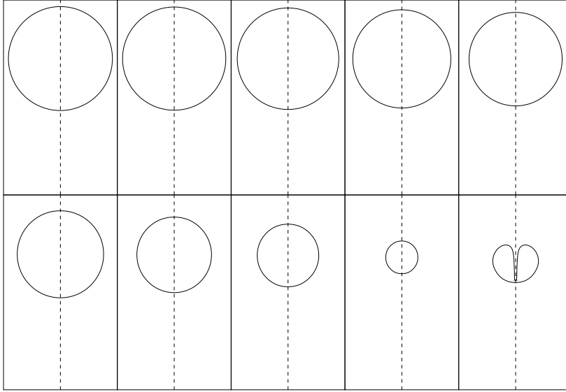
FIGURE 10. Time evolution of a bubble collapsing near a wall at high Reynolds number. The wall is along the bottom side of the box. Not all the simulation domain is shown. Interframe time is 0.243. Re = 29.906 , \alpha = 2.023 , \beta = 2.625 .
