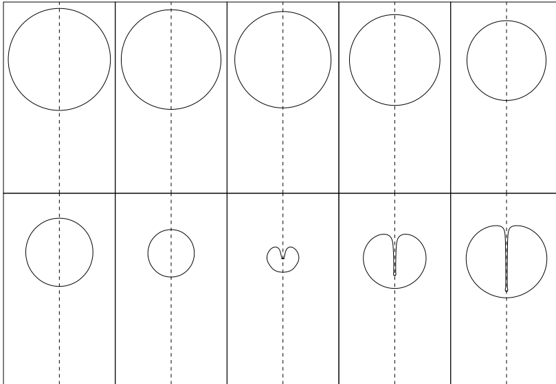
FIGURE 11. Time evolution of a bubble collapsing near a wall at intermediate Reynolds number. Interframe time is 0.303. Re = 24.519 , \alpha = 2.023 , \beta = 2.625 .
