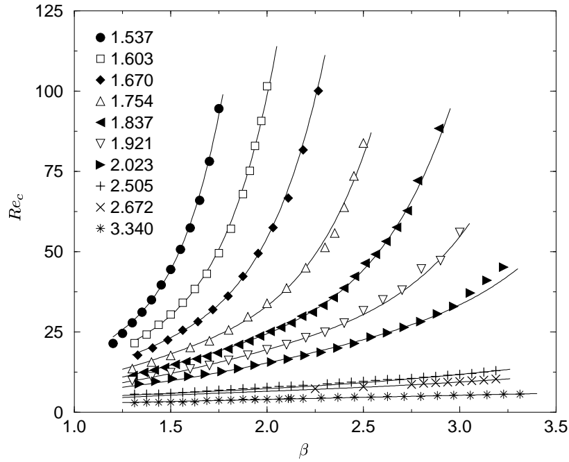
FIGURE 17. Value of the critical Reynolds number Re_c as a function of the relative distance to the solid wall \beta . Each curve corresponds to a different value of the relative initial radius \alpha (indicated in the legend).
