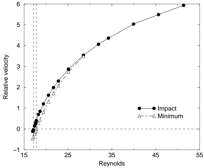
FIGURE 16. Relative impact velocity and minimum of the relative velocity as a function of the Reynolds number. Taking as critical Reynolds number the value of the Reynolds for which the minimum relative velocity is zero gives a good approximation of the Reynolds number for which the jet impact velocity is zero. \alpha = 1.754 , \beta = 1.5 .
