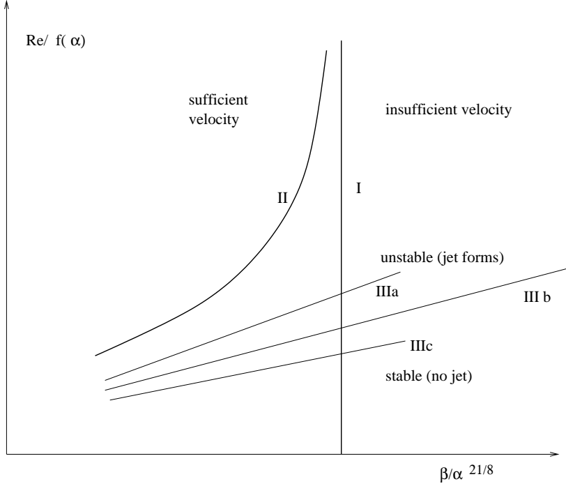
FIGURE 21. A graphical summary of our scaling theory. Curve I is the asymptotic limit at small viscosity, separating a region where the velocity of the jet is too small for impact from a region of large enough velocity. With viscosity, the separation appears as curve II. Jet formation is possible if there is instability, it occurs above curves IIIa,b,c. However these curves are not scaling with \beta , thus each \beta yields a different curve. From our numerical results, there is good reason to assume that all curves of type III are below curve II, so the stability condition is not relevant.
