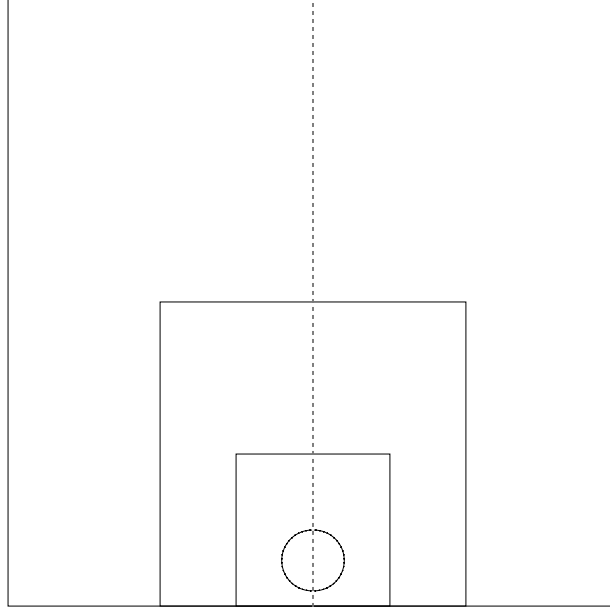
FIGURE 9. Example of the hierarchy of grids used to deal accurately and efficiently with large variations in bubble radius.
