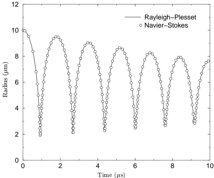
FIGURE 4. Free radial oscillations of a bubble of 5 \mu\text{m} equilibrium radius.
