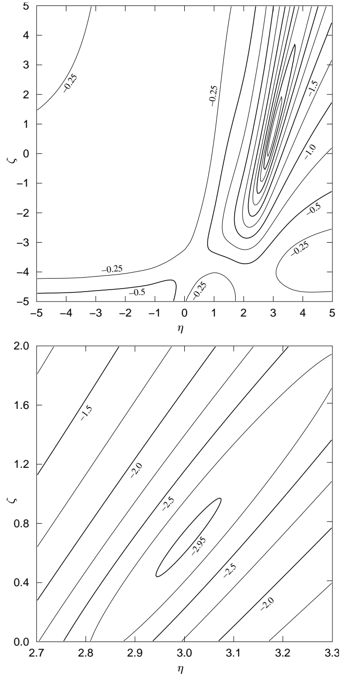
FIGURE 19. Numerical evaluation of the correlation \mathcal{C}(\eta, \zeta) between the rescaled point sets of Figure 17.
