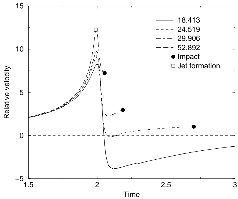
FIGURE 15. Relative velocity between the top and bottom pole of a collapsing bubble as a function of time for various values of the Reynolds number (indicated in the legend). The white squares and black dots mark the time of jet formation (curvature changes sign) and jet impact respectively. \alpha = 2.023 , \beta = 2.625 .
