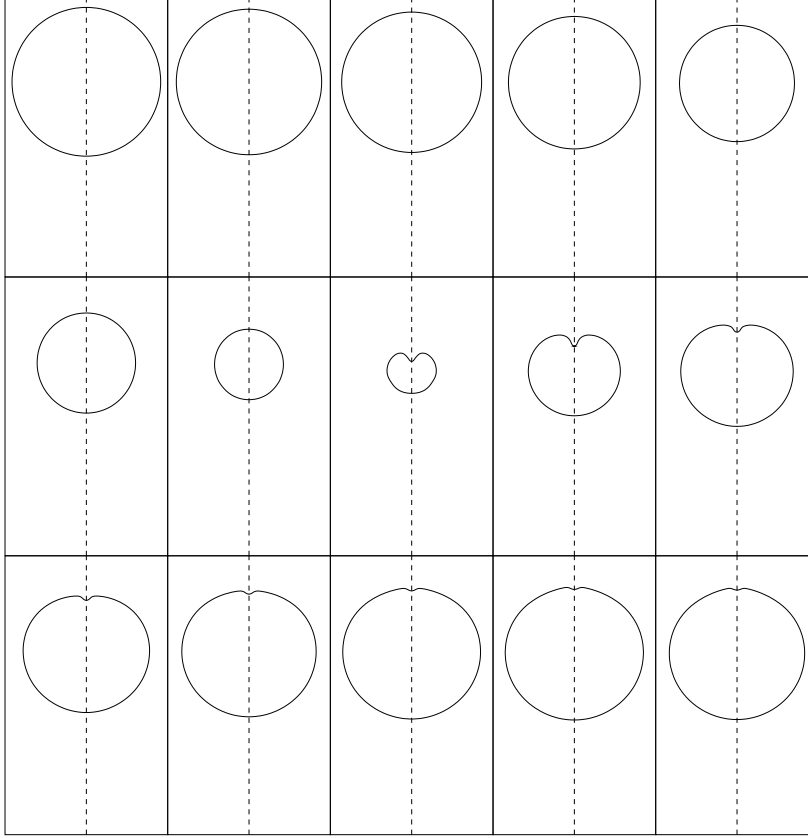
FIGURE 12. Time evolution of a bubble collapsing near a wall at low Reynolds number. Re = 18.413 , \alpha = 2.023 , \beta = 2.625 .
