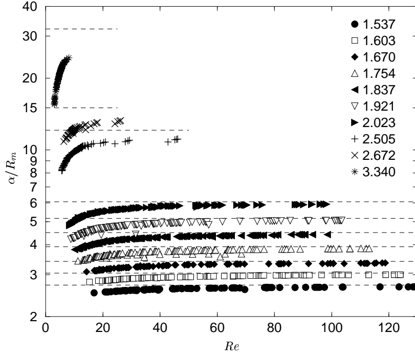
FIGURE 20. Ratio between the maximum (initial) radius \alpha and the equivalent minimum radius R_m as a function of the Reynolds number and for the different values of \alpha indicated in the legend. Theoretical values in the inviscid case given by equation (5.5) are represented by the dashed lines.
