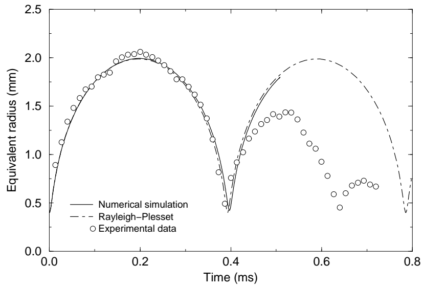
FIGURE 7. Temporal evolution of the equivalent radius of the bubble as given by experimental measurements, numerical simulation and the Rayleigh-Plesset equation.
