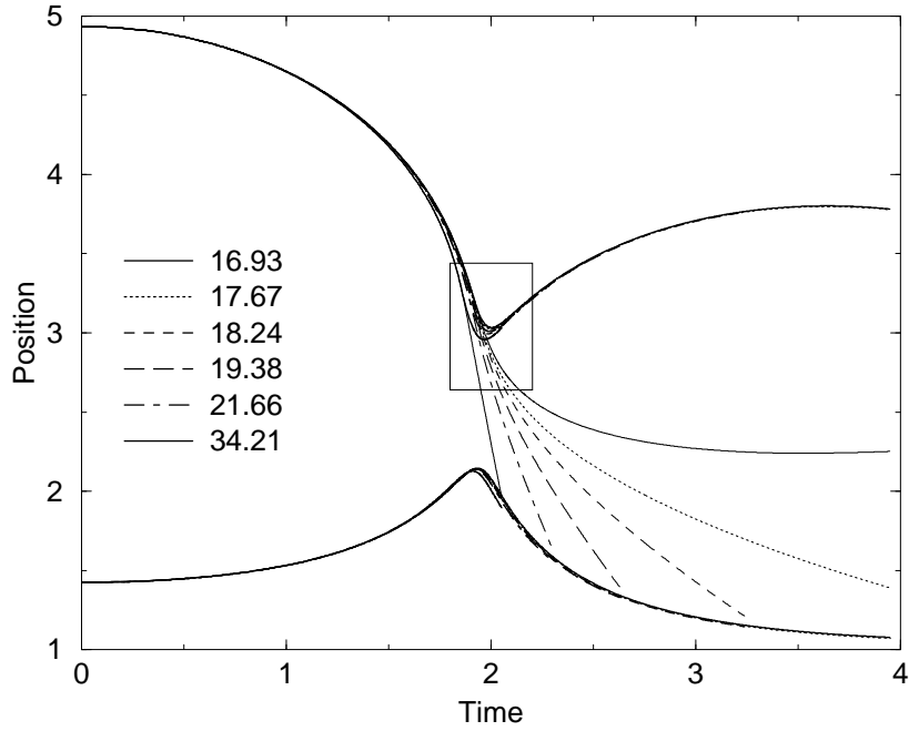
FIGURE 13. Time evolution of the position of the poles as a function of the Reynolds number indicated in the legend. \alpha = 1.754 , \beta = 1.5 .
