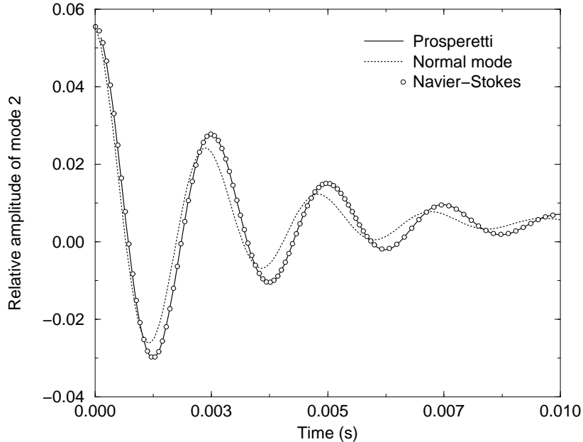
FIGURE 5. Temporal evolution of the second mode of deformation of a slightly ellipsoidal bubble set in a liquid initially at rest.
