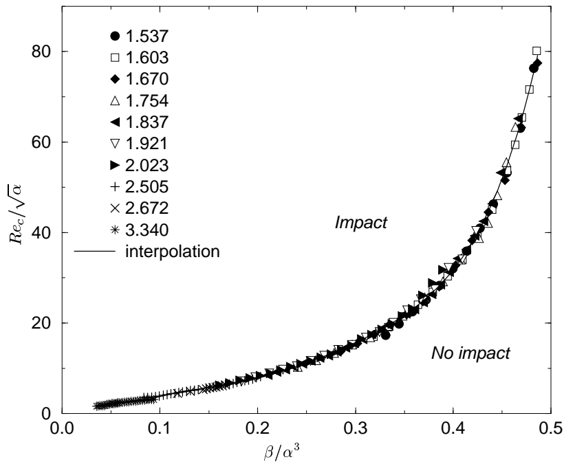
FIGURE 18. Rescaled version of Figure 17. The black line is an interpolating polynomial.
