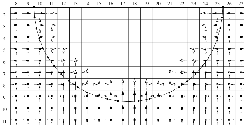
FIGURE 2. Mesh and discretisation of the velocity and pressure fields. The marker points and the connecting cubic splines are represented. The light arrows are extrapolated values of the velocity field. The squares indicate the location of the pressure nodes where the pressure equation is solved.
