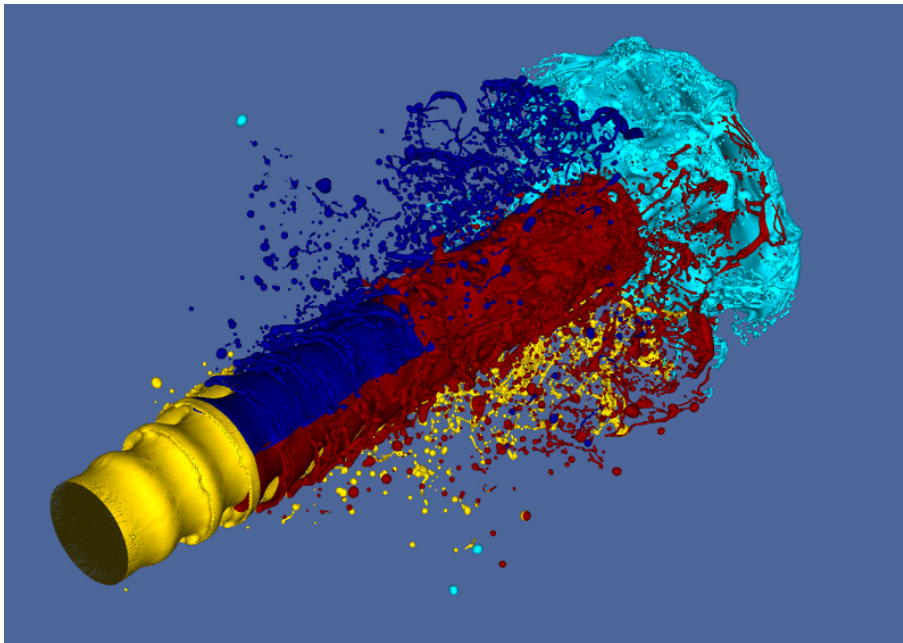
Figure 4. Load-balanced domain decomposition for jet atomisation.
