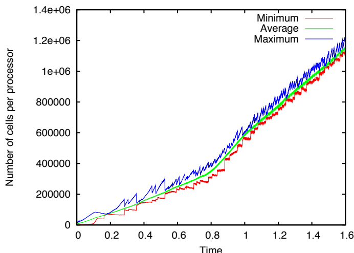
Figure 5. Number of elements per processor as a function of time. Parallel adaptive simulation on four processors with load-balancing.
