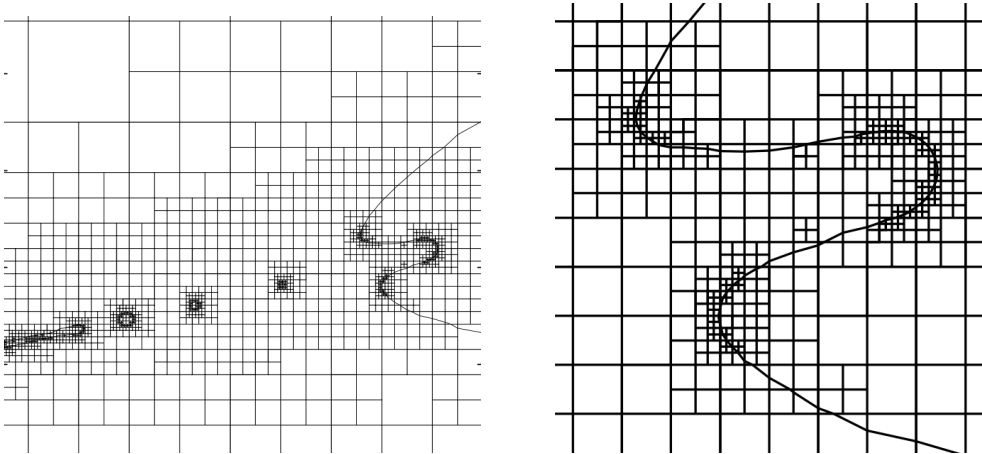
Figure 9. Typical quad-tree grid used to describe the formation of the jet after the droplet has merged with the liquid layer. The criterion for refinement is the curvature of the interface.
