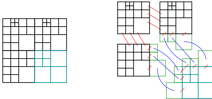
Figure 2. Sketch of parallel domain decomposition on two processors within Gerris. Left: leaf cells colored according to processor number. Right: corresponding structure. The four quadtrees making up the domain are shown, together with “stitches” (red), ghost cells (green), and parallel boundary conditions (blue).
