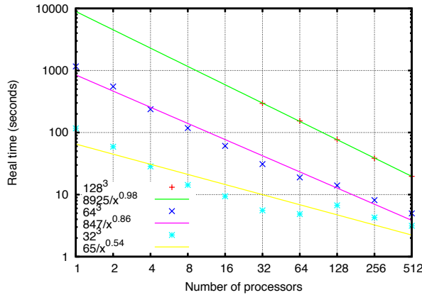
Figure 6. Total computation time as a function of the number of processors for the lid-driven cavity parallel benchmark. IBM supercomputer.
