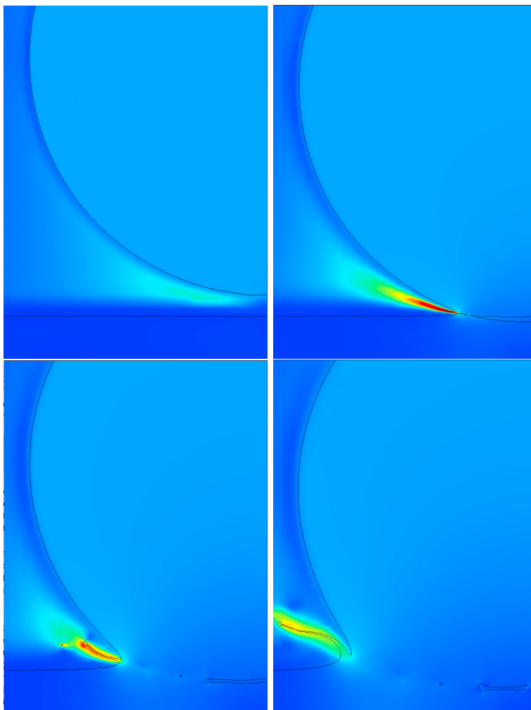
Figure 8. Snapshot of 2D axisymmetric numerical simulation of a droplet impacting on a thin liquid film using Gerris. The color map indicates the velocity norm.
