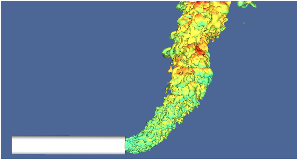
Figure 12. Three dimensional representation of the water/oil interface of a plume generated by the oil leak. Fr = 10 . In colors, the norm of the vertical velocity at the interface. The AMR techniques implemented in Gerris allow capturing the small structures generated by the turbulence of the flow at the tube exit while keeping a relatively low total number of nodes in all the computational domain when compared with an uniform mesh.
