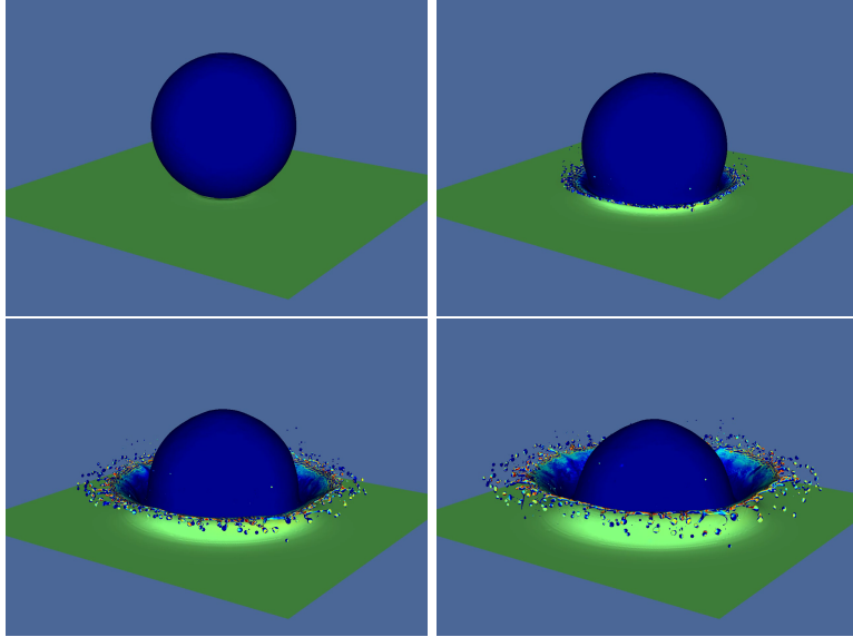
Figure 7. Snapshot of a 3D numerical simulation of droplet impact on a thin liquid film using Gerris. The fluids in the film and in the droplet are the same but have been colored differently in the simulation to illustrate their distribution along the dynamics.
