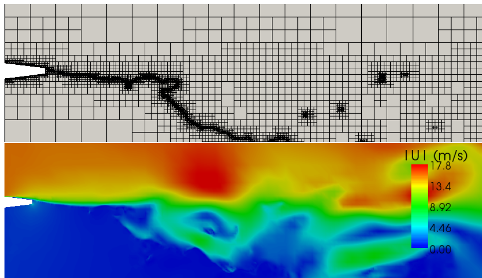
Figure 11. Adaptive mesh (top) and velocity field (modulus) of the flow near the injector. The mesh is adapted at the interface for an accurate representation of the interface. The important velocity gradients induced in the gas phase are also accurately captured by applying dynamically adaptive criteria.
