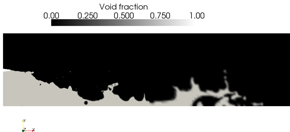
Figure 10. Void fraction field in the whole simulation domain (8x2 cm). Near the injector, a large level of refinement is used in order to capture the effect of the small disturbances on the primary atomization zone. The right boundary of the domain is placed further downstream in order to avoid any influence of the boundary conditions on the flow near the injector. In this region, a low level of refinement is used which has related a significant save of computational time.
