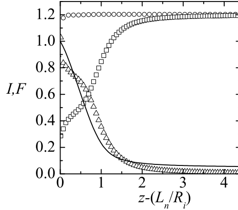
FIG. 7. Axial distribution of the total intensity (circles) and the contributions associated with the bulk conduction (triangles) and the surface convection (squares) calculated by the proposed method for the experimental case with Q = 0.5 ml/h. The shape of the meniscus jet (solid line) is also plotted to show where the transition between conduction and convection of charges takes place.
