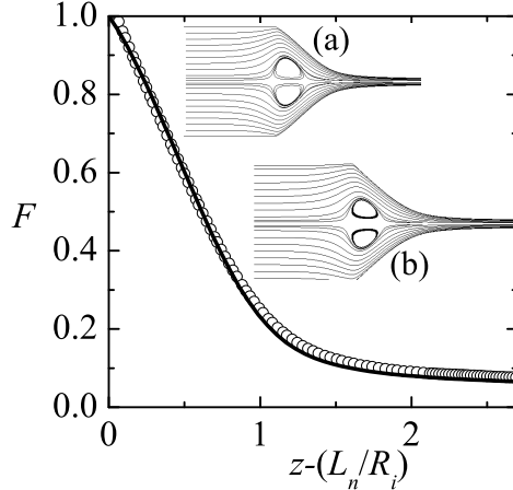
FIG. 4. Free surface position and streamlines calculated with the tracking interface technique [solid line and (a)] and VoF method [symbols and (b)] for C = 0.18 , \beta = 10 , \alpha = 15.3 , \chi = 10 , and v_e = 0.02 .
