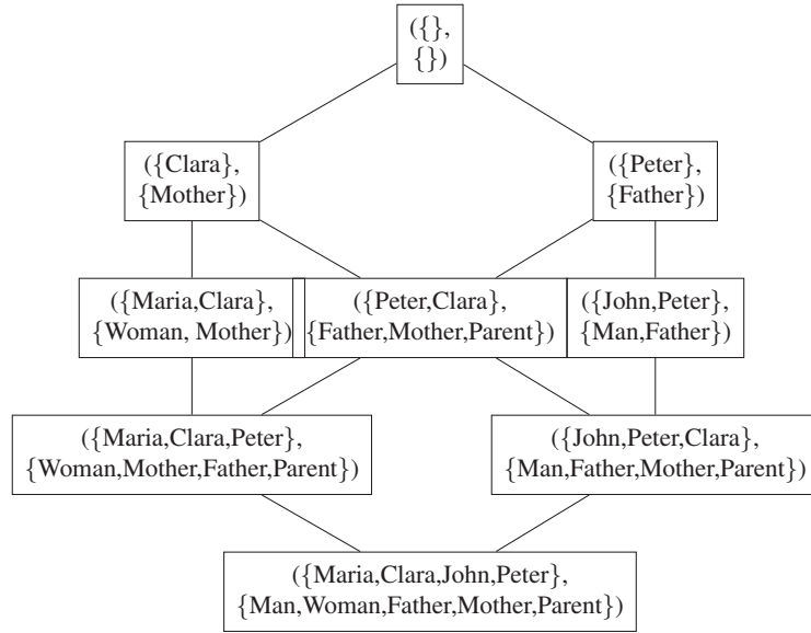
Fig. 1. Lattice \mathcal{L}_{\text{NII}}
