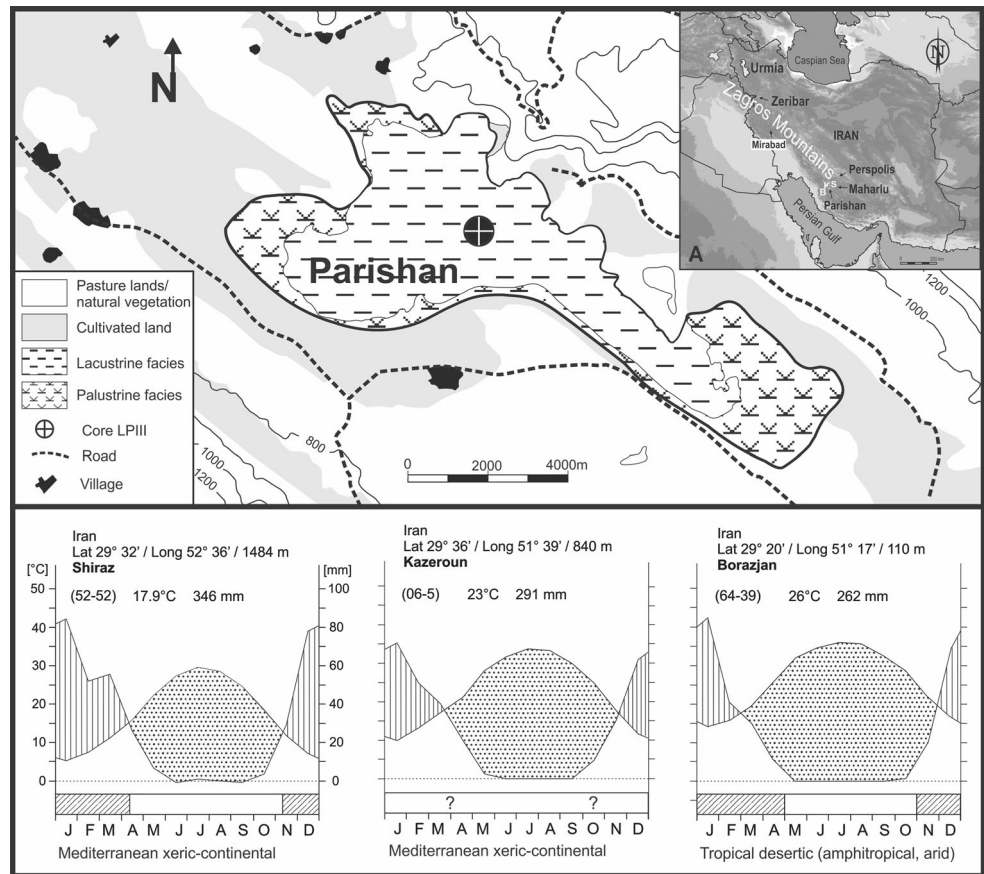
Fig. 1 Sketch map of the Parishan wetland and its surrounding lands with the position of the study core (LPIII). Climate diagrams of Shiraz (S in the inset map), Kazeroun, and Borazjan (B in the inset map) are based on data released by Iran Meteorological Organization
