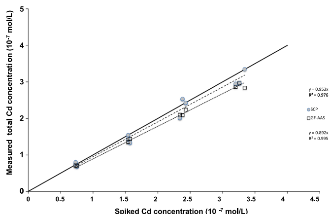
Fig. 3. Comparison of the SCP and GFAAS total measured metal with the real spiked concentration.
