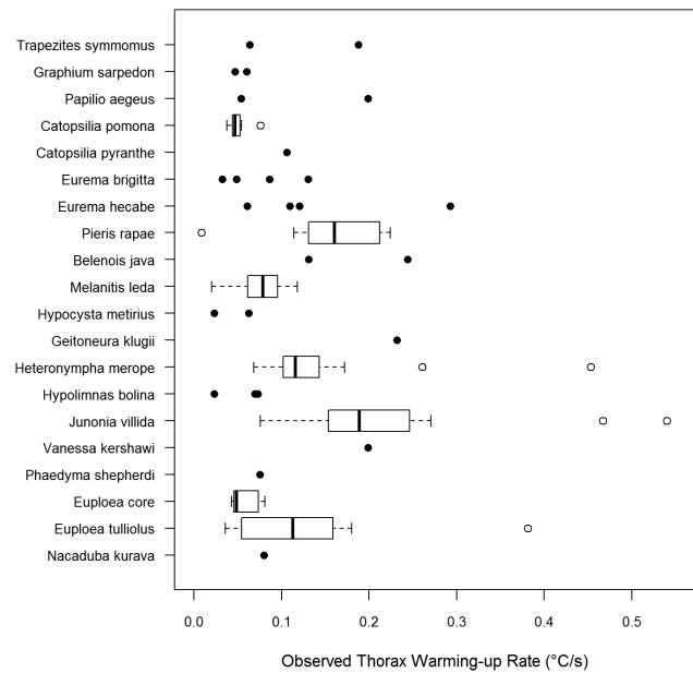
Fig. 3. Warming up speeds at 26°C for all tested Australian butterfly species. Symbols as in Fig. 2.
