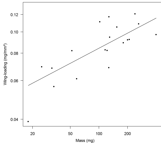
Fig. 9. Wing loading according to mass in 19 Australian butterflies. Trapezites symmomus is omitted; its wing loading is 0.524 mg/mm 2 and its mass is 340 mg. Both scales are logarithmic. The fitted allometric function is y = 0.030x^{0.225} .
