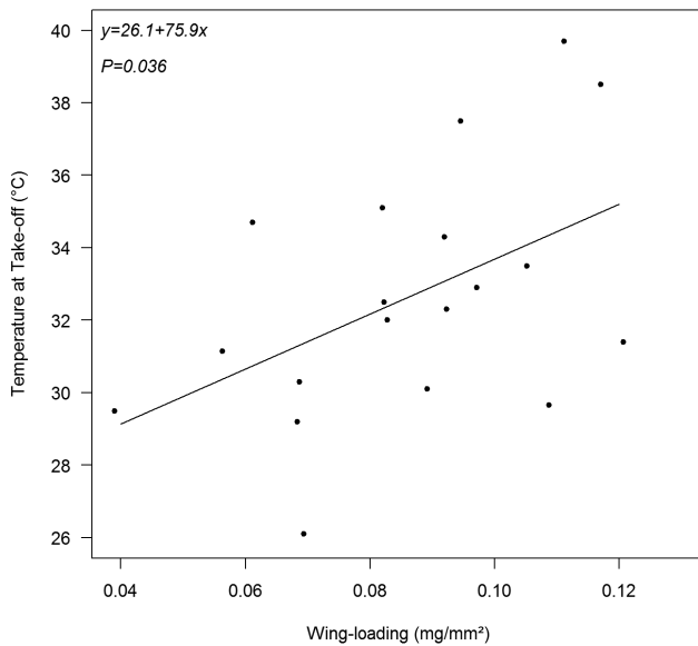
Fig. 8. Temperature at take-off according to wing loading for the 19 tested species ( Trapezites symmomus is omitted; its wing loading is 0.524 mg/mm 2 and median thorax temperature at take-off was 33°C); dots indicate median values per species. The line indicates the linear correlation for all depicted points.
