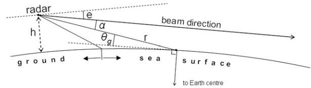
FIG. 3. Radar geometry.
