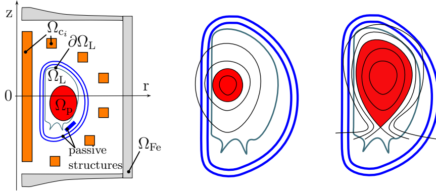
Figure 1: Left: Geometric description of the tokamak in the poloidal plane. Middle and right: Sketch for characteristic plasma shapes. The plasma boundary touches the limiter (middle) or the plasma is enclosed by a flux line that goes through an X-point (right).
