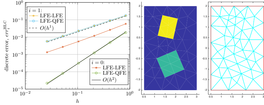
Figure 3: Left: The suboptimal convergence rate for \psi^{HLC} in L^2 can be improved if we use quadratic finite elements (LFE-QFE) instead the linear finite elements (LFE-LFE) in (20) for the auxiliary variable u . Right: The computational domain \Omega and the coarsest mesh, with the subdomains D (yellow), the domain where we evaluate the error and the domain C (green) the support of the source term.
