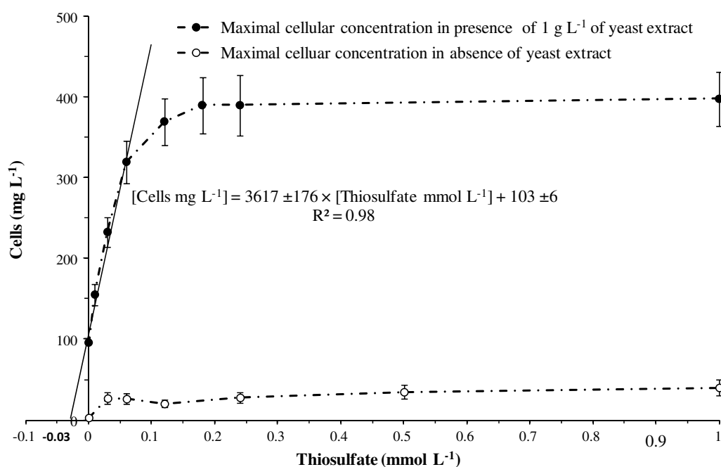
Fig. 3 Maximum cellular concentrations versus thiosulfate concentrations. In the absence of yeast extract, maximal biomass is obtained with glucose (25 mmol L -1 ) as energy source. The cultures were performed in triplicate in serum bottles after nine subcultures under the same conditions. In the presence of yeast extract at 1 g L -1 , maximal biomass is obtained with glucose (60 mmol L -1 ). These cultures were performed in triplicate in bioreactor
