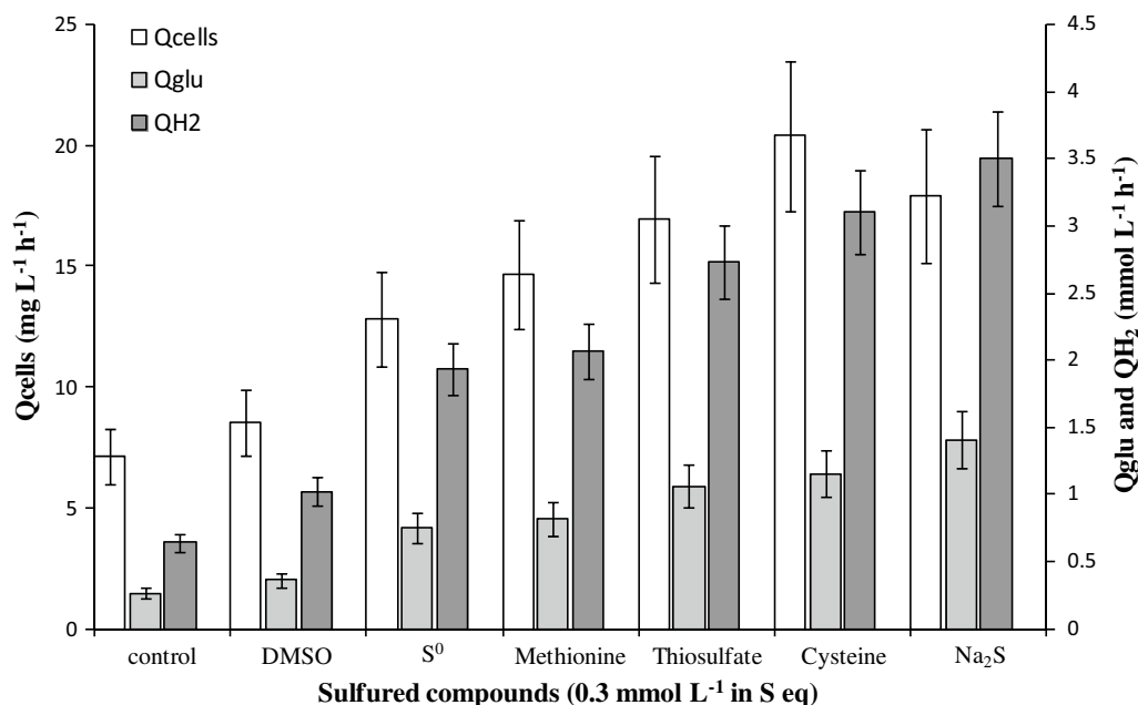
Fig. 1 Comparisons of different sulfured nutriment on Thermotoga maritima cultures. All sulfured compounds were added at the rate of 0.3 mmol L -1 sulfur equivalent in a medium containing glucose (25 mmol L -1 ), yeast extract (1 g L -1 ), and salts (see “Methods” section). DMSO, S 0 , and Na 2 S meant dimethyl sulfoxide, elementary sulfur, and sodium sulfide, respectively. Productivities of cells (Q cells ), and of hydrogen (Q H 2 ), and consumption of glucose (Q glu ) were calculated during the growth phase (after 14.5 h of incubation). All batch cultures were performed in triplicate in serum bottles. The control corresponded to T. maritima grown without adding the sulfured compounds
