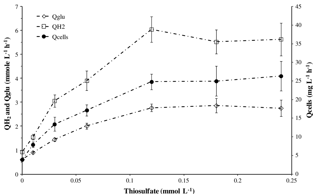
Fig. 4 Glucose consumption and hydrogen and cells productivities versus thiosulfate concentrations. Hydrogen productivities (QH 2 ) and glucose consumptions (Qglu) were expressed in mmol per liter of medium and per hour. T. maritima cells productivities (Qcells) were expressed in mg per liter of medium and per hour. These fermentation parameters were calculated during the growth phase from fermentation runs performed in bioreactor (in triplicate). For all fermentations, culture medium contained glucose (60 mmol L -1 ) and yeast extract (1 g L -1 )
