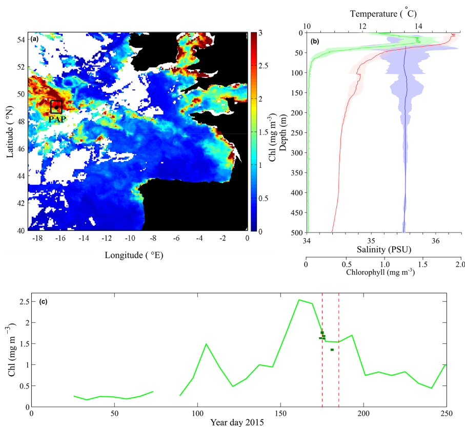
Figure 1. Surface chlorophyll concentration ( \text{mg m}^{-3} ) at the PAP site; (a) PAP study region (black box) overlain on 9 km Aqua MODIS satellite chlorophyll for 18–25 June 2015. (b) Average vertical temperature, salinity and chlorophyll profiles measured at the PAP site (red, blue and green lines, respectively) and the standard deviation (light shading) of CTD deployments coinciding with MSC deployments. (c) Temporal change in surface chlorophyll ( \text{mg m}^{-3} ) over the PAP study region based on 8-day, 9 km Aqua MODIS satellite data. Gaps in data are due to cloud cover. Vertical red lines indicate start and end of sampling period, and dark green squares are discrete measurements made from the CTD at depths of 5–10 m.
