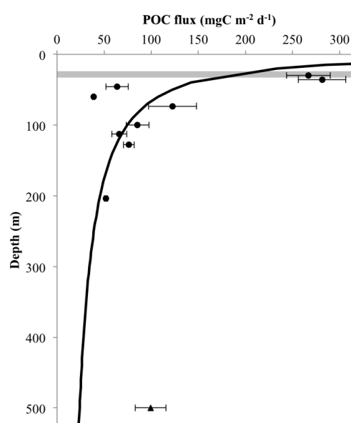
Figure 4. Flux of POC ( \text{mg C m}^{-2} \text{d}^{-1} ) with depth at the PAP site. POC fluxes of fast-sinking particles measured in June 2015 at the PAP site via deployment of MSCs. Error bars relate to replicate filters per sample. A power-law curve was fitted to the data (black line), Y = 194.9 (X / \text{MLD})^{-0.71} ( R^2 = 0.42 , p = 0.060 , n = 9 ), excluding the point at 500 m (triangle) which is likely due to non-steady-state conditions. The grey shaded area indicates the mixed layer depth over the study period.
