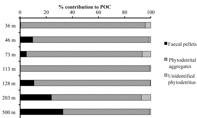
Figure 2. Composition of fast-sinking POC at each measured depth horizon. The percent (%) contribution of faecal pellets (black), phytodetrital aggregates (hatched) and unidentified phytodetritus (grey) to the total mass of fast-sinking POC collected in MSCs at each depth horizon. See Table 1 for numbers of particles in each category.
