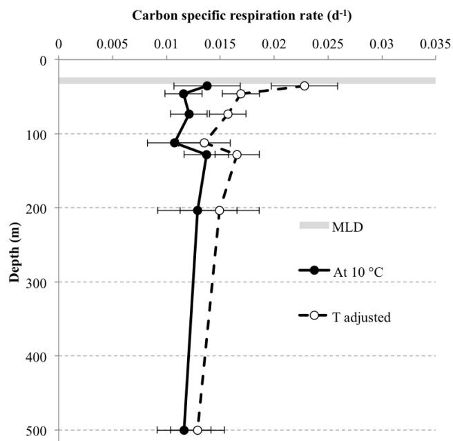
Figure 7. Carbon-specific respiration rates ( \text{d}^{-1} ) for aggregates collected at depth. Rates adjusted to the in situ temperature ( T ) are shown by the dashed black line (open circles). Grey shading shows the range in mixed layer depth over the study period, and error bars represent standard errors.
