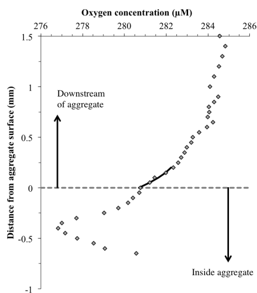
Figure 5. Example oxygen profile (µM) through a phytodetrital aggregate collected at 46 m depth. Measurements were made with microsensors in steps of 50–100 µm, with negative values reflecting the distance into the aggregate from the surface. The solid black line shows the model fit used to calculate the oxygen flux in the diffusive boundary layer.
