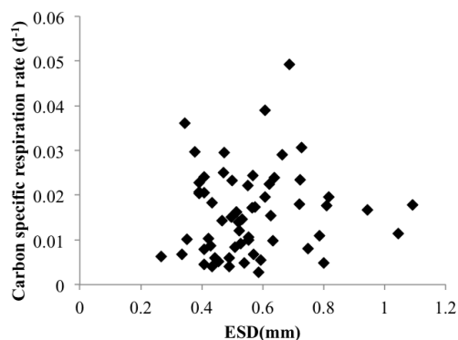
Figure 8. Carbon-specific respiration rates ( \text{d}^{-1} ) of phytodetrital aggregates collected at depth. Data have been adjusted for in situ temperatures (see text).
