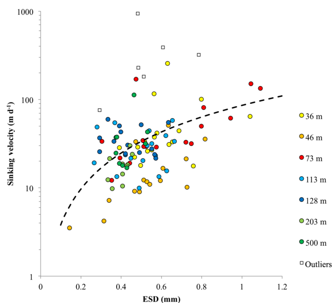
Figure 3. Relationship between sinking velocity ( \text{m d}^{-1} ) and equivalent spherical diameter (ESD, mm) of phytodetrital aggregates. The depth from which aggregates were sampled is shown by the colour of circles (36 m = yellow, 46 m = orange, 73 m = red, 113 m = light blue, 128 m = dark blue, 203 m = light green and 500 m = dark green). Note the log scale on the y axis. We apply a power-law fit for between sinking velocity and aggregate ESD (dotted line Y = 85.8X^{1.4} ). A total of six outliers (black open squares), defined as being outside 2 standard deviations from the mean, were excluded from the power-law fit.
