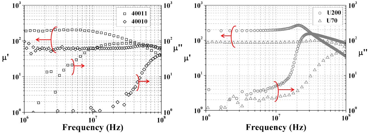
Figure 5. Measured complex permeability: ESL 40010® and 40011® ferrites sintered at 950°C/2h and 885°C/3h ( b=4\text{ mm} , c=6\text{ mm} and h=108\text{ }\mu\text{m} ), U70 and U200 home-made ferrites sintered at 980°C/2h ( b=5\text{ mm} , c=14\text{ mm} and h=1.5\text{ mm} )
