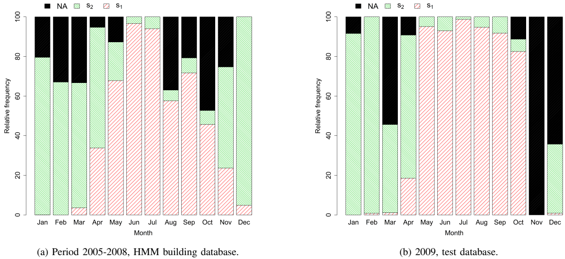
Fig. 6. State distribution per month for a typical seasonal cycle: state s_1 is represented in red color and s_2 in green color. The black color, named NA, concerns measures whose state is not estimated (one least missing values).
