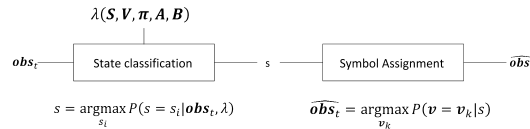
Fig. 7. Time series reconstruction from HMM classification. Signal \widehat{\mathbf{Obs}} is reconstructed from original observation \mathbf{Obs} thanks to the M symbols.
