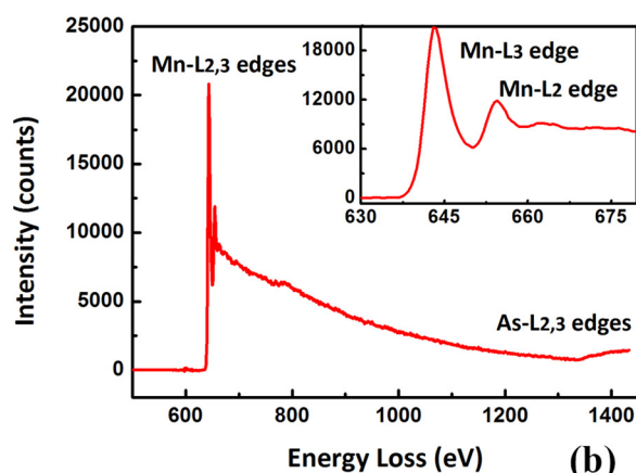
FIG. 2. (a) Bright field image of selected grain in the plan-view sample of MnAs/GaAs(001) at RT at low magnification of 60 000 \times , and diffraction pattern acquired at zone axis of [\bar{2}201] in the inset. (b) Electron energy loss near edge spectrum of the crystal at RT.
