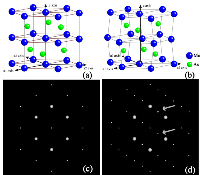
FIG. 1. Atomic structure of hexagonal \alpha -MnAs (a) and orthorhombic \beta -MnAs (b). Diffraction patterns of \alpha -MnAs at \langle 2\bar{2}01 \rangle zone axes in (c) and that of \beta -MnAs at the zone axis in (d). The diffraction patterns are simulated by PDF software.
