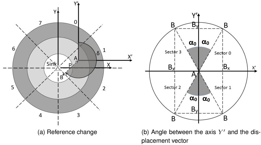
Figure 7 – Angle displacement
