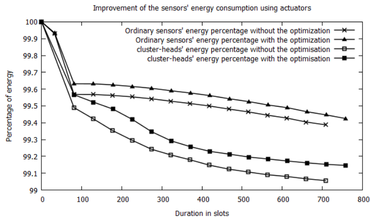
Figure 10 – Improved of the power consumption using actuators a mobile sensor. It would be also interesting to integrate data aggregation techniques to minimize the number of messages circulating in the network. Authentication and security are also important issues in this kind of network.
