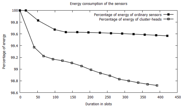
Figure 9 – Energy consumption of ordinary sensors and cluster-heads
