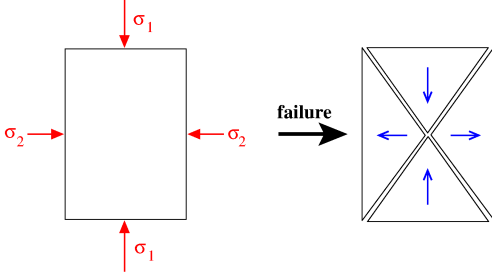
FIG. 13. Left: Principle of a biaxial test. Right: Schematic representation of the response of the material after failure.
