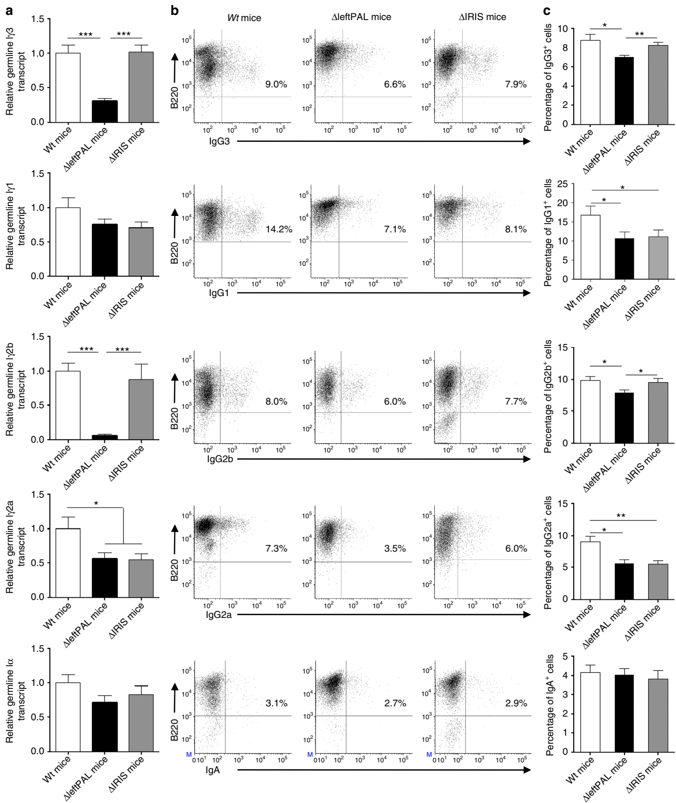
Figure 4 | Influence of the 3'RR palindrome on GLT and CSR. (a) GLT in B splenocytes of \Delta leftPAL, \Delta IRIS and wt mice. Cells were stimulated with LPS \pm IL-4, \text{INF}\gamma and TGF \beta for 2 days. I\gamma 1 - C\gamma 1 , I\gamma 2a - C\gamma 2a , I\gamma 2b - C\gamma 2b , I\gamma 3 - C\gamma 3 and I\alpha - C\alpha GL transcription was investigated by real-time PCR. Mean \pm s.e.m. of six independent experiments with one mouse (8–12 weeks old, male and female). * P < 0.05 and *** P < 0.0001 (Mann-Whitney U -test for significance). Values were normalised to GAPDH transcripts. (b) CSR in B splenocytes of \Delta leftPAL, \Delta IRIS and wt mice. Cells were stimulated with LPS \pm IL-4, \text{INF}\gamma and TGF \beta for 3 days. Cells were then labelled with anti-B220-APC antibodies and anti-IgG _1 -, anti-IgG _{2a} -, anti-IgG _{2b} -, anti-IgG _3 - and anti-IgA-FITC antibodies. One representative experiment out of six (one mouse per experiment) is shown (8- to 12-week-old mice, male and female). (c) Mean \pm s.e.m. of six independent experiments of CSR with one mouse (8–12 weeks old, male and female). * P < 0.05 and ** P < 0.001 (Mann-Whitney U -test for significance).
