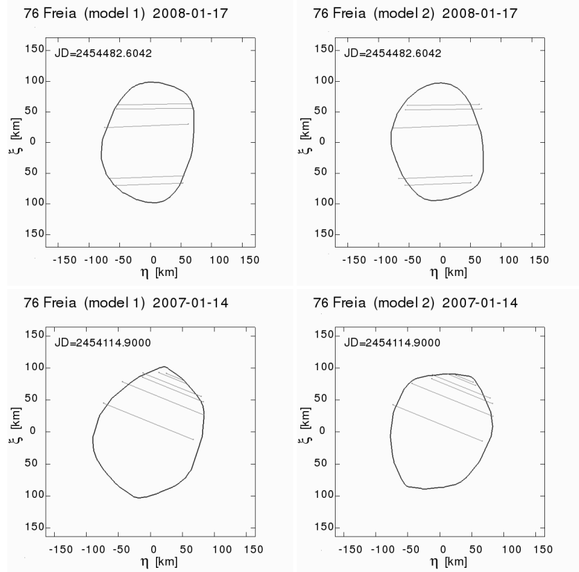
Fig. 17. Occultation chords with both scaled shape models for asteroid (76) Freia. Two occultation events.
