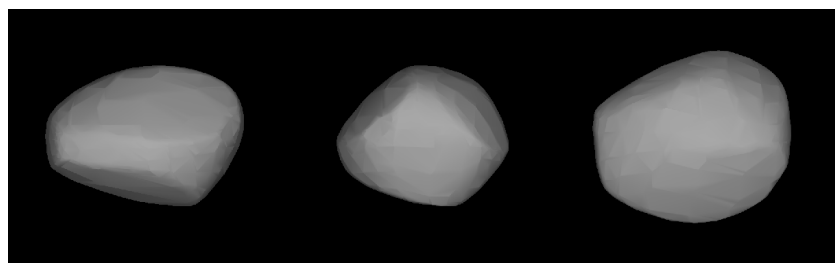
Fig. 10. Shape model “2” of (417) Suetia.
