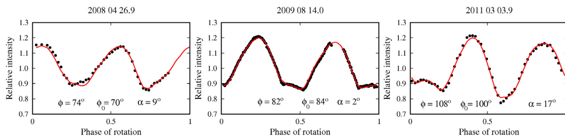
Fig. 11. Observed vs. modelled lightcurves for (435) Ella. The rms residual of the fit was 0.0153 mag.
