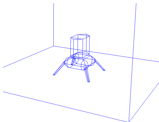
Figure 4. Luna-Glob simulation model
