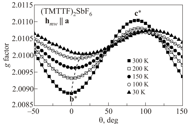
Fig. 1. A representative g -factor angular dependence for (\text{TMTTF})_2\text{SbF}_6 at different temperatures when the static magnetic field is applied perpendicular to the \mathbf{a} axis. The evolution of the position of the g_{b^*} is indicated by a dashed line.
