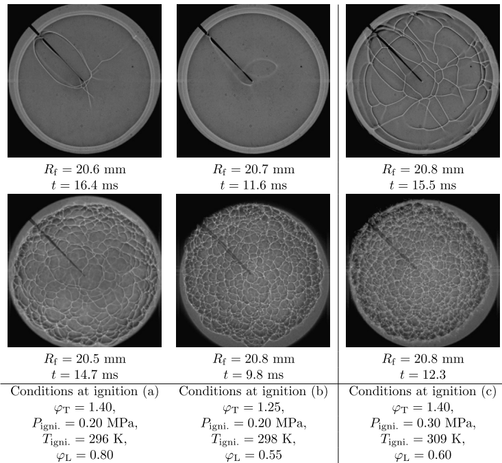
Fig. 10. Sequences of shadowgraphy images of aerosol flames compared with gaseous flames.
