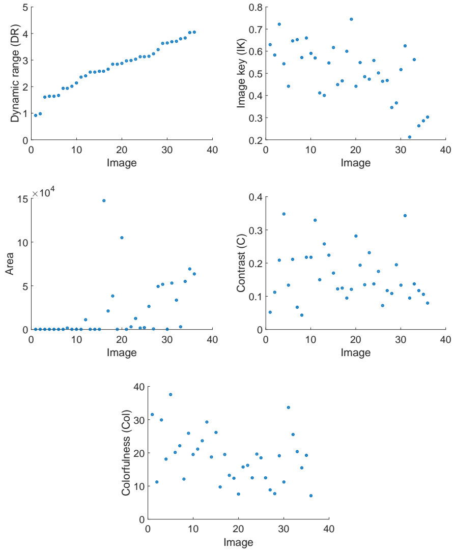
Figure 2: Image features: pixel-based DR (top-left), IK (top-right), Area (middle-left), Contrast (middle-right) and Colorfulness (bottom), all sorted by pixel-based DR.
