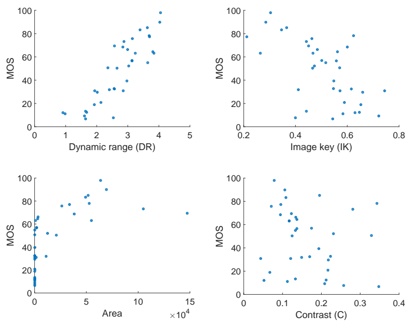
Figure 6: Achromatic MOS across the four objective measures (top-left to bottom-right): pixel-based DR, IK, Area and Contrast.
