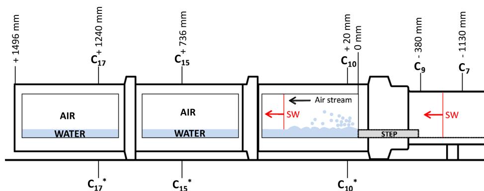
Fig. 1 Scheme of the T200 experimental section and principles of the experiment. The C_7 and C_9 pressure sensors allow for the determination of the Mach number of the incident shock wave. The C_{10} , C_{15} ,
