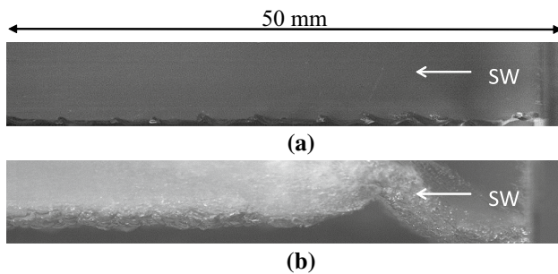
Fig. 3 Magnified images extracted from experiments conducted with a water layer having a depth of 10 mm driven by shock waves with Mach numbers of 1.11 (a) and 1.43 (b). SW represents the propagation direction of the incident shock wave
