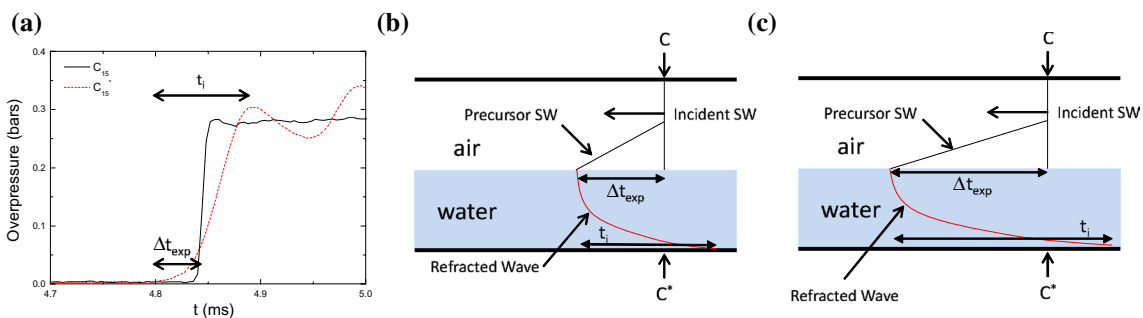
Fig. 5 a Pressure signals for comparing the pressure increase behind the planar incident shock wave in air (black line) and the compression wave in water (red dashed line). \Delta t_{exp} represents the time gap between the two waves at the same location, and t_i represents the duration of the pressure increase in water. b, c Diagrams showing the
