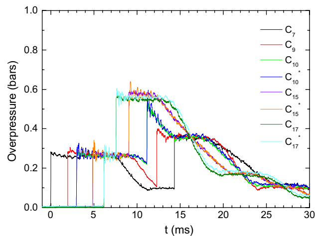
Fig. 4 Pressure signals recorded throughout the experimental apparatus both in air and water
