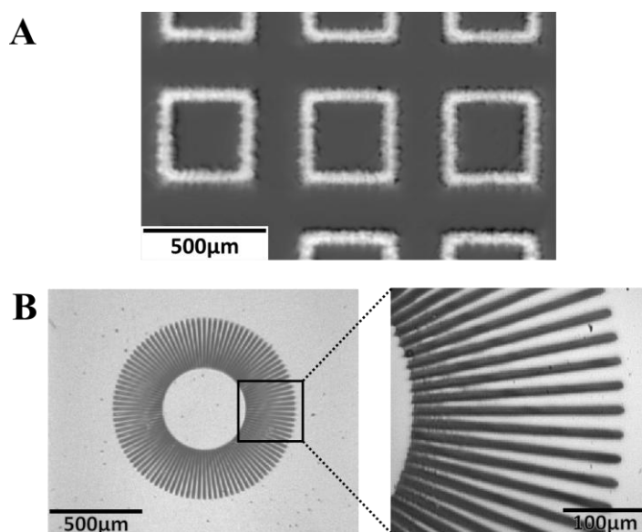
Figure 6. Optical microscopy images of PNIPAM hydrogel patterns. The patterns are obtained with a 8 Watt UV lamp through photomasks. Square patterns with 50 μm-wide and 2.5 μm-thick walls are grafted on glass surface (A). 6 μm-wide and 250 nm-thick patterns are grafted on silicon wafer (B).
