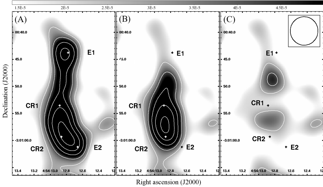
Fig. 7. VLA 1.4 GHz maps obtained by tapering the A+B-array data set with a Gaussian of FWHM = 30 \text{ k}\lambda . The crosses indicate the positions of the radio detections identified in Fig. 4. Panel (A) includes all the emission between E1 and E2. In panel (B) the CC models of E1 and E2 were subtracted from the data before the tapering and cleaning procedure. Panel (C) shows what is left when CR1 and CR2 are also subtracted from the data. The gray-scale has units of \text{Jy beam}^{-1} , and the corresponding contours are drawn at 2, 3, 4, 5 and 6 times the 1\sigma noise level of 14 \mu\text{Jy beam}^{-1} . The dimensions of the beam are 5.27'' \times 5.12'' at a position angle of -88:25 (panel (C), top right corner).
