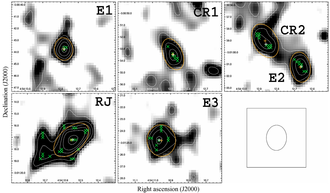
Fig. 5. Detail of the six radio sources located within the sub-mm emission region in Fig. 4. The white radio contours are drawn at 2, 3, 4, 5, 6 and 8 times the 1\sigma noise level of 10.34 \mu\text{Jy beam}^{-1} . The radio peak positions ( S_{\text{pk}} ) listed in Table 1 are indicated with white plus-symbols. The green crosses correspond to the positions of the clean components in each source model. Orange plus-symbols and ellipses represent the center and \text{FWHM} of the best fitting Gaussian for each source. A scaled version of the radio beam ( 2.14'' \times 1.71'' ) at a position angle of -1^\circ.43 is included in the bottom right panel .
