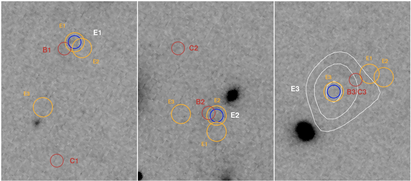
Fig. 15. Analysis of the lensing nature of E1, E2 and E3 with the lens model MFINAL. The orange circles indicate the image positions predicted after tracing each of the three radio sources independently into the source plane and lens them back into the image plane. The radius of the circles correspond to 0.3'' . The rest of the labels are the same used in Fig. 8.
