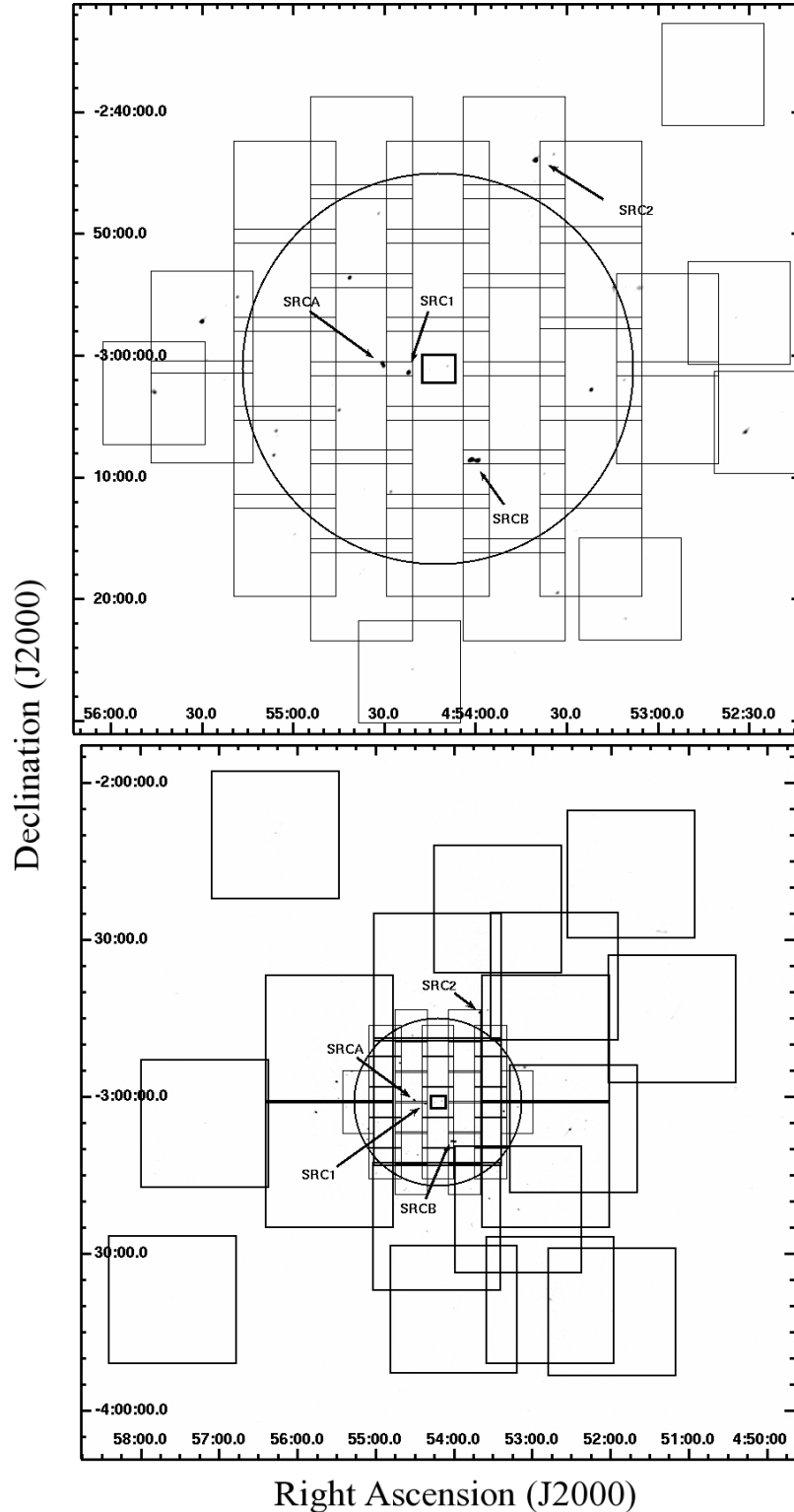
Fig. 2. VLA 1.4 GHz maps centered in the core of the cluster MS0451.6-0305. The maps were produced using the visibilities of the central 10\text{ k}\lambda region of the UV-plane only, to enhance the source visibility. The facets used during the selfcalibration of the cluster data are indicted with boxes, while the circle represents the VLA FWHM primary beam ( 0.5^\circ at 1.4 GHz). The central bold box corresponds to the target region mapped in Fig. 4. The brightest sources in the field are indicated with labels. Top panel: 1^\circ \times 1^\circ map produced with the A-array observations. Each box is 8.4' \times 8.4' . Bottom panel: 1.5^\circ \times 1.5^\circ map produced with the B-array observations. The big boxes (used in the first step of the selfcalibration procedure) are 27.8' \times 27.8' in size, whereas the small boxes (used in the second step) are 6.8' \times 6.8' .
