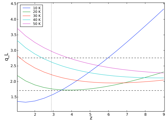
Fig. 11. Change of the parameter q_L with redshift for different characteristic dust temperatures. The horizontal dashed lines indicate the minimum and maximum value of q_L found in the SMG sample studied by Kovács et al. (2006). The dotted vertical line indicates the position of z = 2.9 .
