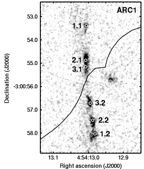
Fig. 13. Detail of the optical arc as seen in the HST image. The circles indicate the positions of the three sets of mirror images listed in Table 6.
