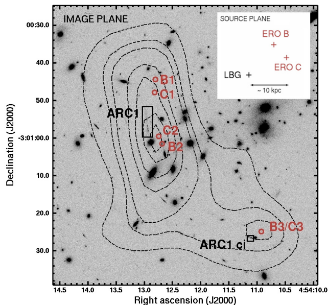
Fig. 1. Summary of the results presented in Borys et al. (2004). SCUBA 850 \mu\text{m} contour map of SMM J04542-0301 superimposed upon a HST image of the center of the cluster MS0451.6-0305. Highlighted with rectangles are an optical arc (ARC1) and its counter image (ARC1 ci), produced by a LBG at z_{\text{spect}} = 2.911 . The red circles indicate the positions of five NIR sources that have been interpreted as multiple images produced by two EROs (ERO B, lensed as B1/B2/B3, and ERO C, lensed as C1/C2/C3) at z_{\text{model}} = 2.85 \pm 0.1 . Assuming z = 2.9 for both the LBG and the EROs, their predicted positions in the source plane would be located within a region of \sim 10 kpc, suggesting that they constitute a merger.
