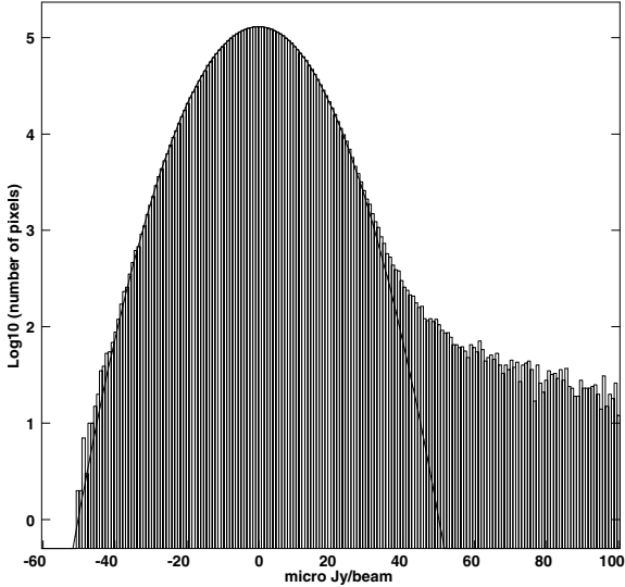
Fig. 3. Histogram of the A+B array clean map produced using R = 0.6 . The black curve is the best Gaussian fit to the noise peak, while the positive excess on the right side is due to source emission. The good agreement between the fit and the data in the negative side of the Gaussian indicates that the noise of the map is well behaved, making faint detections more reliable.
