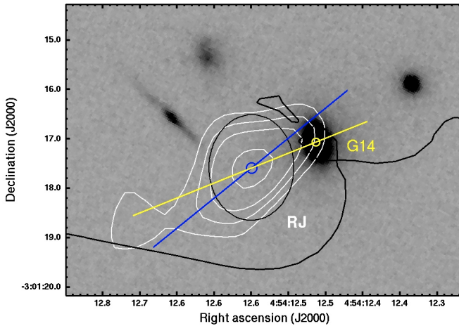
Fig. 9. Detail of the HST image in the region of RJ, including the critical curve at z = 2.911 predicted by the lens model describe in Sect. 4.1 (black line). The contours correspond to the \sim 2'' resolution radio map presented in Fig. 4. The radius of the circles show the estimated positional uncertainties: 0.1'' for RJ (see Table 1) and \sim 0.08'' (half a pixel) for G14. The blue line indicates the approximate orientation of the major axis of the radio source. For comparison, the yellow line shows the orientation of the RJ centroid respect to the galaxy G14. The black ellipse indicates the beam size of the radio map ( 2.14'' \times 1.71'' ) at a position angle of -1^\circ 43' .
