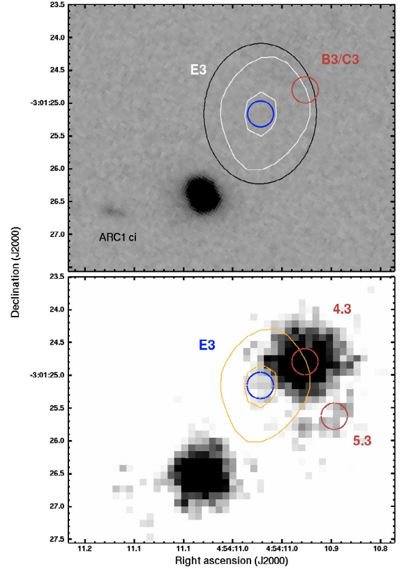
Fig. 14. Detail of the source E3, including its radio contours as presented in Fig. 4. Top panel: HST image of the region, including the positions of the counter images of the optical arc (ARC1 ci) and the ERO pair (B3/C3) reported by Borys et al. (2004) . Bottom panel: K′ band image of the region, indicating the constraints used in the lens model (4.3 and 5.3). The radius of the circles show the estimated positional uncertainties: \sim 0.20'' for the K′ band sources (astrometric error for the standard stars quoted in Takata et al. 2003 ), 0.2'' for E3 (see Table 1) and \sim 0.08'' (half a pixel) for the optical sources. The black ellipse indicates the beam size of the radio map ( 2.14'' \times 1.71'' at a position angle of -1^\circ 43' ).
