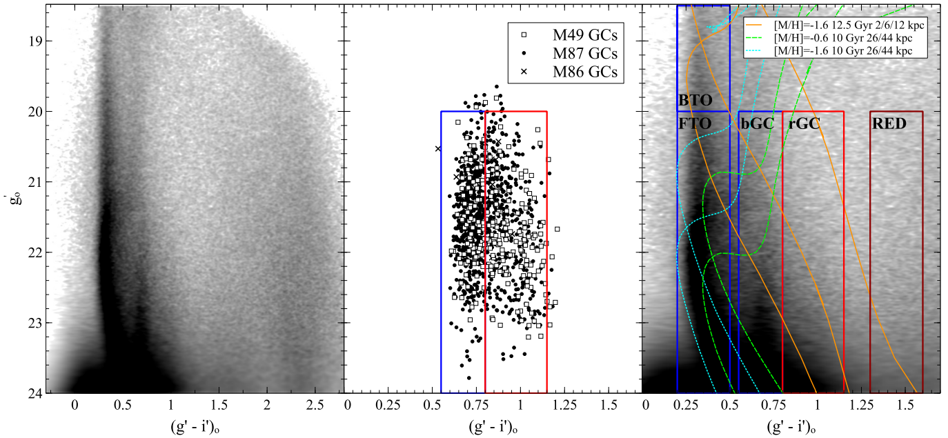
Figure 2. (left) g'_o , (g' - i')_o Hess diagram for all point sources that satisfy the \Delta i' criterion (Figure 1) and have 18.5 < g'_o < 24.0 . The colors and magnitudes for all sources have been smoothed by a value of the combined photometric errors and a constant value. (center) g'_o , (g' - i')_o color-magnitude diagram for radial velocity-confirmed Virgo cluster GCs; the colored boundaries show the adopted color and magnitude criteria used for blue GCs (bGCs) and the red GCs (rGCs). (right) The g'_o , (g' - i')_o Hess diagram for point sources overplotted with Marigo et al. (2008) isochrones with representative age/metallicity values appropriate for stars in the Milky Way halo at distances of 2–16 kpc (orange lines), and for stars expected to be in the Sagittarius dwarf galaxy (cyan and green lines) incorporating a spread in both the distance and metallicity; see text for details. The boxed regions are the locations of the (from top left to bottom right) bright MW halo turnoff stars (BTO), faint [Sgr] turnoff stars (FTO), the blue globular cluster region (bGC), the adjoining red globular cluster region (rGC) and the red halo star populations (RED).
