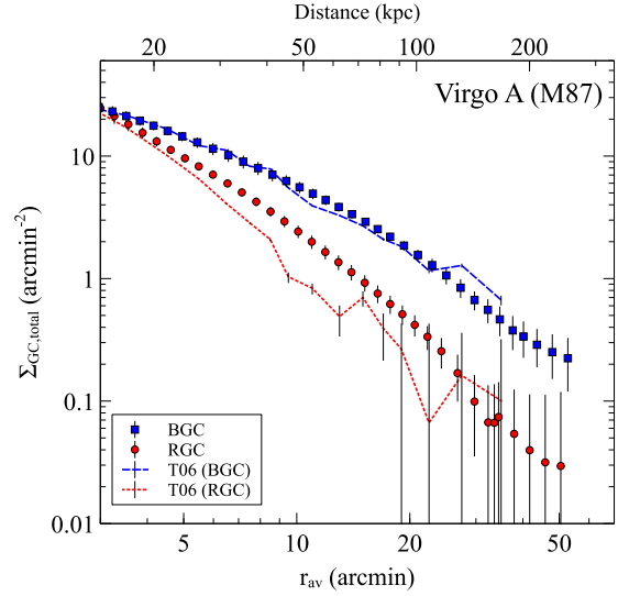
Figure 14. Total number density profiles as a function of average radius r_{av} = r_{maj}\sqrt{1-\epsilon} for the blue (squares; blue in the online version) and red (circles; red in the online version) globular cluster populations for Virgo A(M87), derived from ellipse fits to the adaptive-smoothed maps. Here the plotted number densities \Sigma_{GC,total} have been corrected for those GCs missed in the point-source selection criteria and those objects with g'_o > 24 . The dashed lines show the total GC number densities for the blue and red GC populations from Tamura et al. (2006b) for a region stretching east from M87 towards M59.
