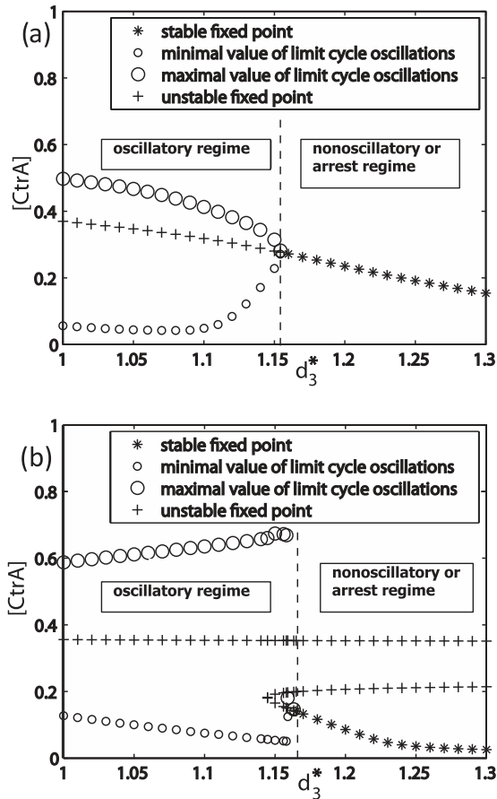
FIG. 4. The two cell cycle arrest scenarios in the weak coupling (a) and strong coupling (b) cases. In case a) the limit cycle shrinks upon approach to the critical value of the degradation constant of DnaA and the transition arises in a continuous fashion. In the strong coupling case b), the limit cycle first expands while an additional branch of unstable fixed points appears. The transition progresses in three steps: limit cycle \rightarrow limit cycle \rightarrow arrest state.
