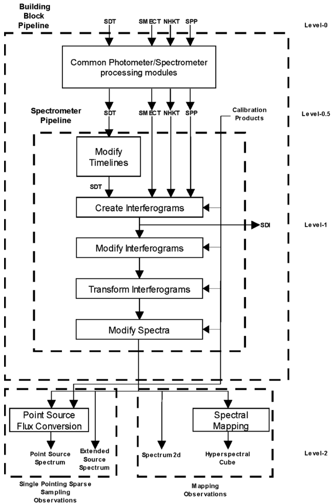
Figure 2. SPIRE FTS data processing block diagram.
