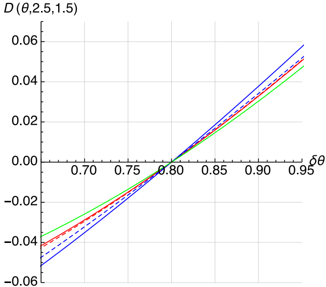
Figure 20. Magnitude difference for a point-like object (green), an elliptical galaxy (red), and a spiral galaxy (blue) convolved with a PSF \mathcal{M}[\theta, 2.5] as a function of the seeing \theta and for two different effective radii, 0''.5 (solid line) and 0''.8 (dashed line), when the extraction is performed in 3'' diameter apertures.
