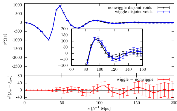
FIG. 2. Same as Fig. 1 for disjoint voids.
