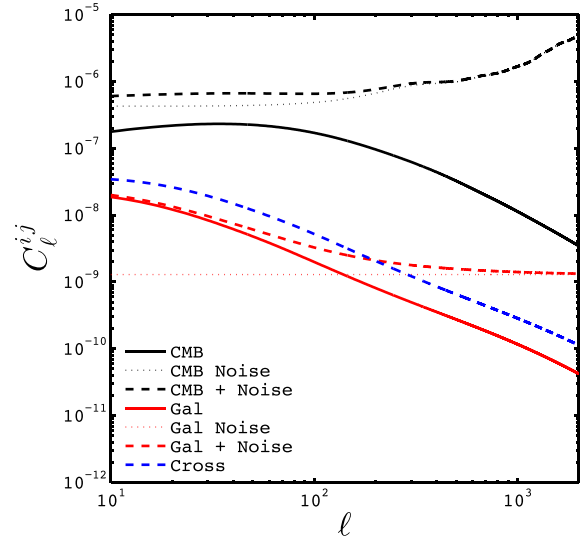
Figure 2. Theoretical predictions for the autospectra ( ij = \kappa_{\text{CMB}}\kappa_{\text{CMB}} and ij = \kappa_{\text{gal}}\kappa_{\text{gal}} ) and cross-spectrum ( ij = \kappa_{\text{CMB}}\kappa_{\text{gal}} ). These are based on RCSLenS specifications for the shape noise \sigma_\epsilon , number density \bar{n} and redshift distributions n(z) . For CFHTLenS, the cross-spectrum is approximately a factor of 2 higher, due to a deeper n(z) .
