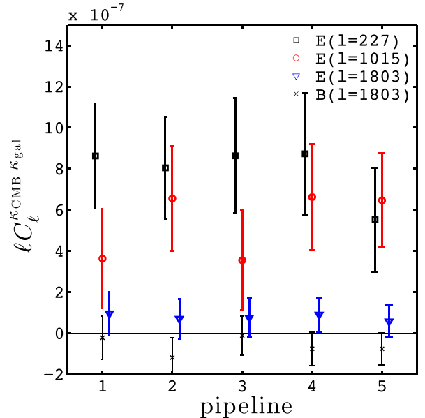
Figure B1. RCSLenS measurements of the \hat{C}_\ell^{K_CMB K_gal} for all pipelines listed in Table 2. E modes are presented for multipoles \ell = 227, 1015 and 1803 in squares, circles and triangles. B modes are shown for the \ell = 1803 with cross symbols. All pipelines are consistent within 1\sigma , however they result in important differences in significance as seen in Table 3.
