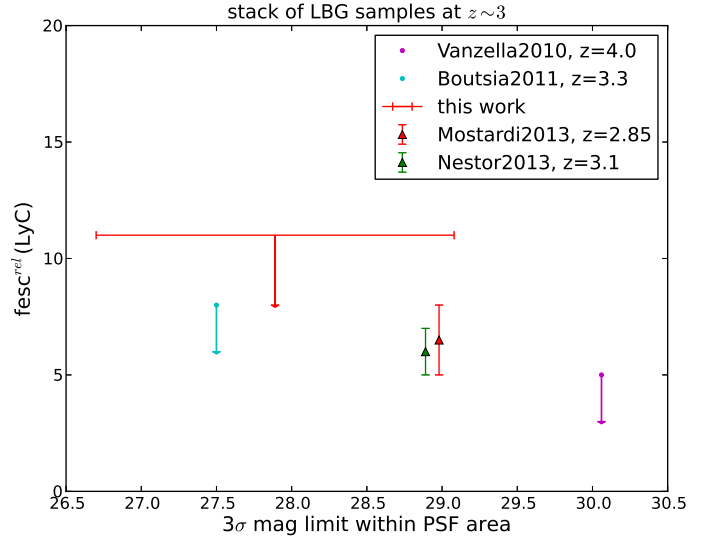
Fig. 11. Relative LyC escape fraction as a function of survey depth. We translate the fesc rel (LyC) estimations in the literature into values corresponding to L_v(1400)/L_v(900) = 5 , where needed. The limits correspond to 1\sigma . The survey depths all correspond to the 3\sigma detection limit in an area equal to the survey PSF seeing. Together with our upper limit (red arrow), we include the upper limits from the stack of Vanzella et al. (2010a) at 3.4 < z < 3.8 (magenta arrow and dot), of Boutsia et al. (2011) at z \approx 3.3 (cyan arrow and dot), and the measurements from the stack of Nestor et al. (2013) at z \approx 3.1 (green triangle) and Mostardi et al. (2013) at z \approx 2.85 for Lyman break galaxies.
