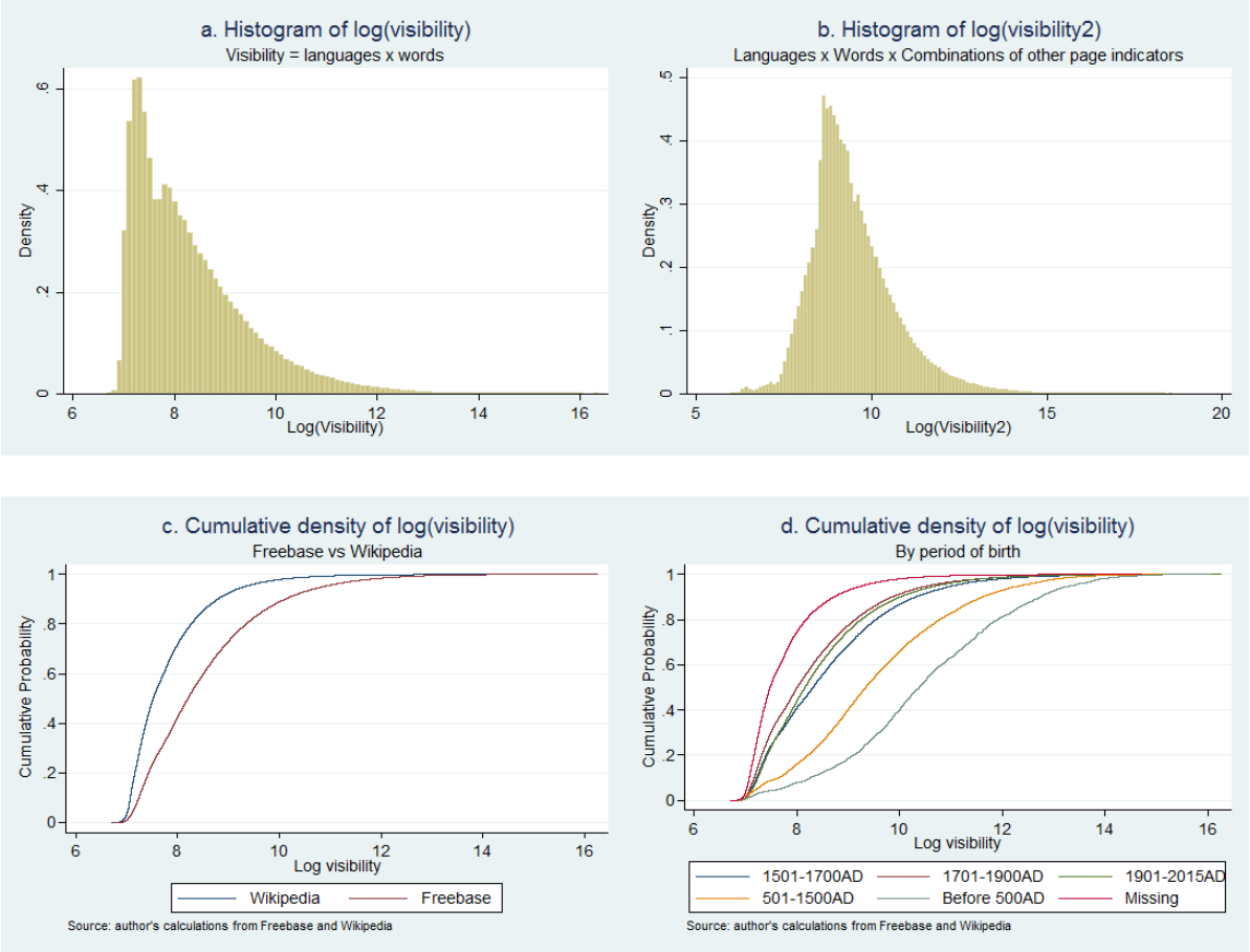
Figure 9: Visibility indices
