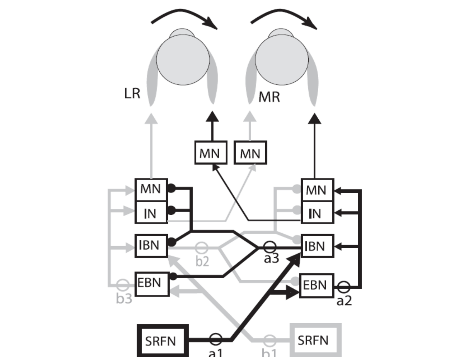
FIG. 10. Scheme by which the saccade-related neurons in the cFN (SRFN) influence the generation of the horizontal component of saccades. See text for additional details. Arrows, excitatory connections; connecting lines ended by a circle, inhibitory connections. The connecting lines have different thickness for clarity purposes.
