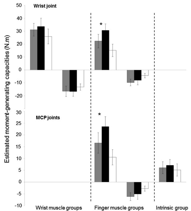
Fig. 4 Estimated muscle moment-generating capacities at the wrist joint level ( upper panel ) and MCP joints level ( lower panel ). Muscles included in the different muscles groups are detailed in Table 1. Non-climbers are in gray , male climbers are in black and female climbers are in white . Asterisk indicates a significant differences between non-climbers and climbers. Flexion and Extension are positive and negative values, respectively. No muscle capacities were presented for the intrinsic muscle group at the wrist joint and for the wrist muscle groups at the MCP joints since these muscles do not cross these respective joints
