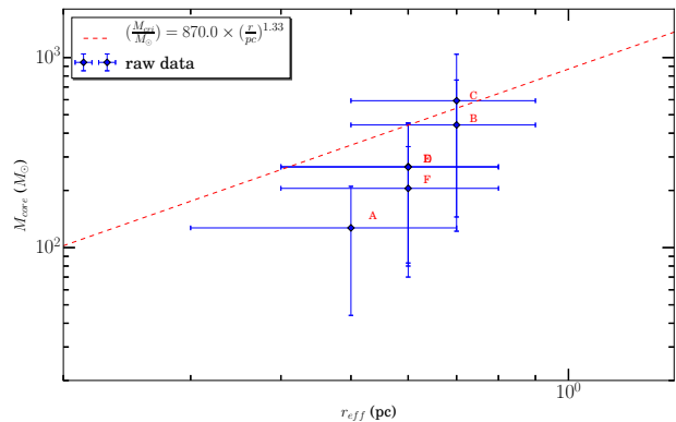
FIG. 6.— Mass-size relationship of the six clumps. The dashed line represents an empirical relation of m(r) = 870 M_{\odot} (r/\text{pc})^{1.33} , which is expected to be as a threshold for forming high-mass stars (Kauffmann & Pillai 2010).
