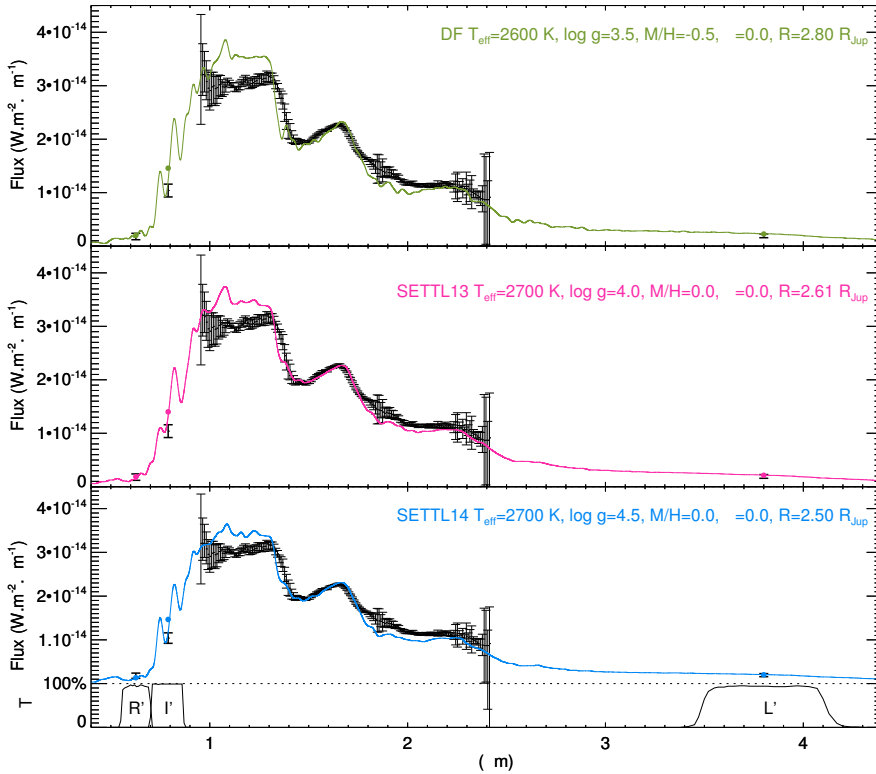
Fig. 14. First version of the PZ Tel B SED (black) compared to best-fitting synthetic spectra for three atmospheric models (see text).
