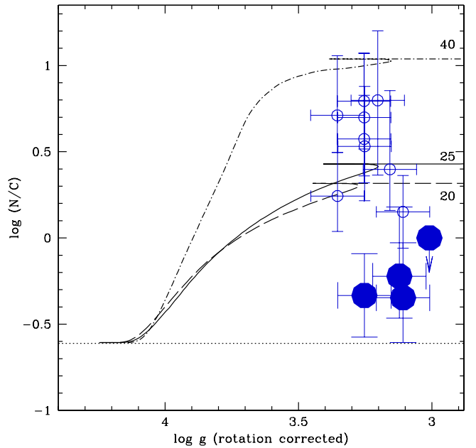
Fig. 2. \log(\text{N}/\text{C}) - \log g diagram for the sample stars (filled circles) and comparison late-type supergiants (open circles). Evolutionary tracks including rotation from Ekström et al. (2012) are overplotted, labeled by initial masses. The dotted line shows the initial chemical composition. For non-rotating models, \text{N}/\text{C} remains at the initial value (dotted line) throughout the main sequence and early post-main sequence phases.
