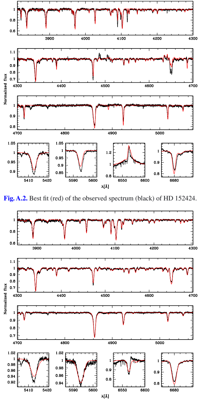
Fig. A.3. Best fit (red) of the observed spectrum (black) of HD 154811.
