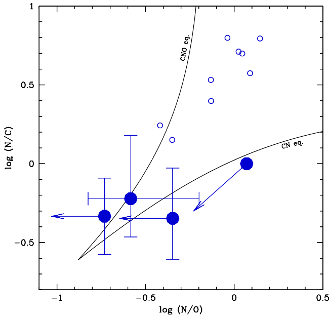
Fig. 3. \log(N/C) - \log(N/O) diagram for the sample stars (filled circles) and comparison late-type supergiants (open circles) from Martins et al. (2015a) . Solid lines indicate the prediction of nucleosynthesis through the partial CN or complete CNO cycle.
